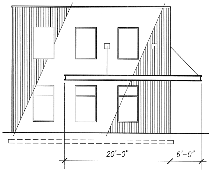
NORTH ELEVATION
