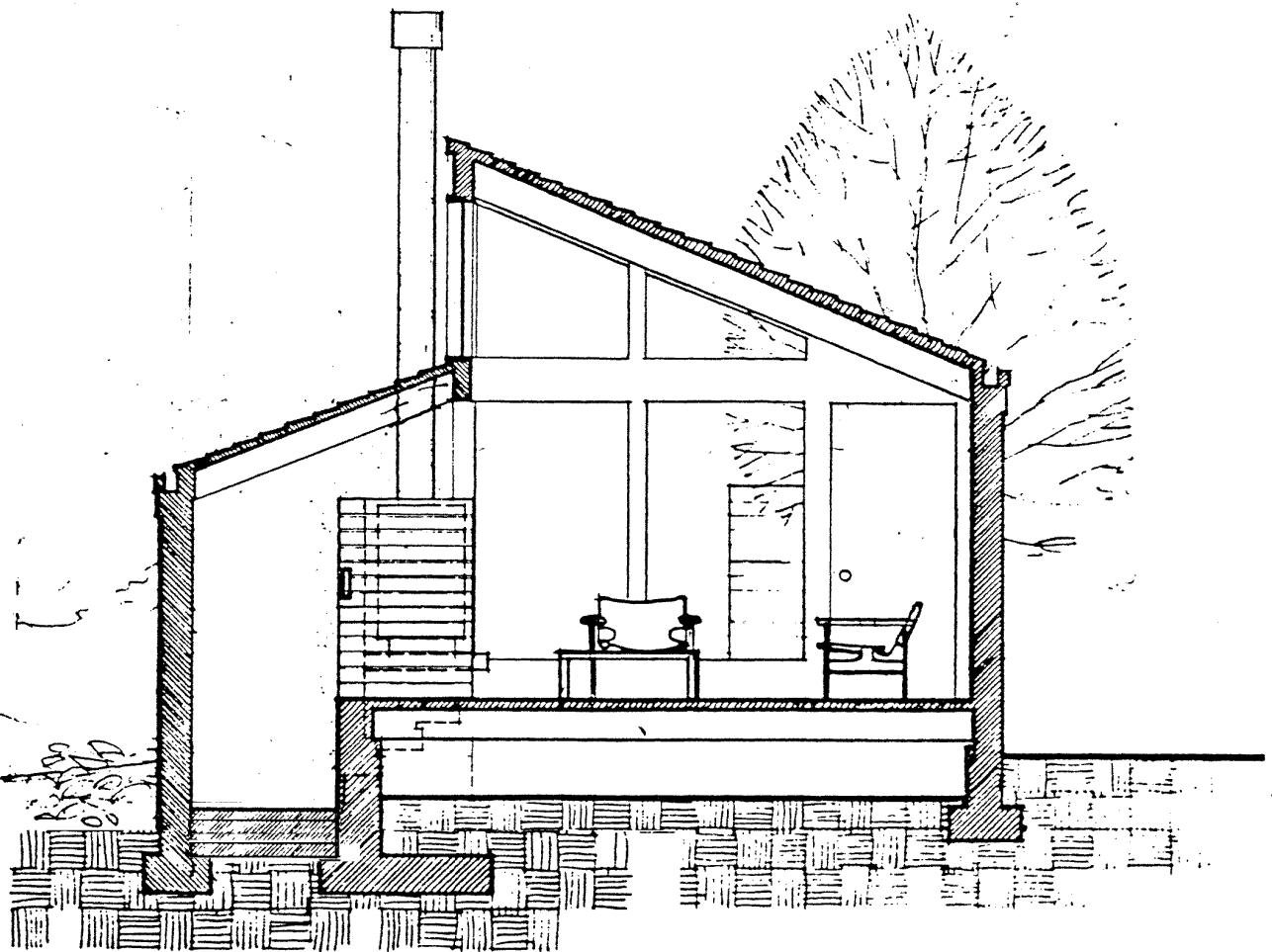
SECTION A-A \frac{1}{4}'' = 1'-0''
