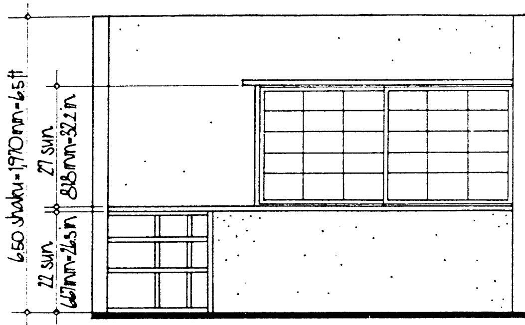
interior elevation of entrance wall
