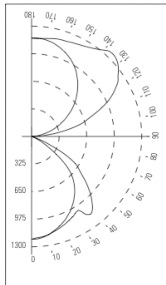
Candlepower Curve
