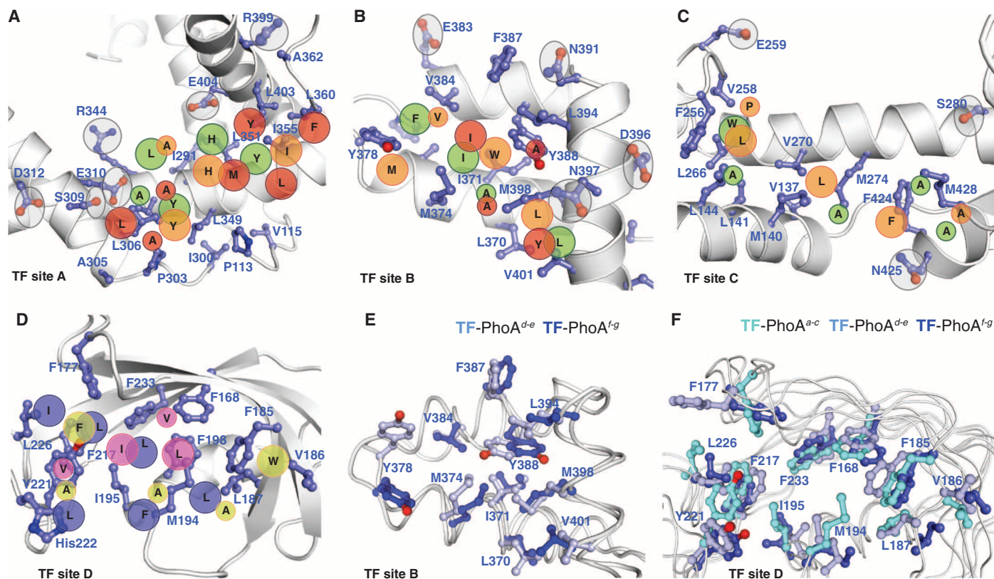
Fig. 6. Substrate recognition conformational plasticity by TF. (A to D) Interaction and recognition patterns of the PhoA sites in the complexes with the three TF molecules. A close-up view of each one of the four substrate-binding sites in TF (labeled TF site A, B, C, and D) is shown, with the backbone in white ribbon and the interacting residues in blue sticks. The position of hydrophobic residues from PhoA sites interacting with TF is projected on the TF structure and denoted as large (for aromatic or Ile/Leu residues) or small (for Ala/Val residues) circles. For clarity, only one TF molecule is shown. The substrate-binding sites A,
