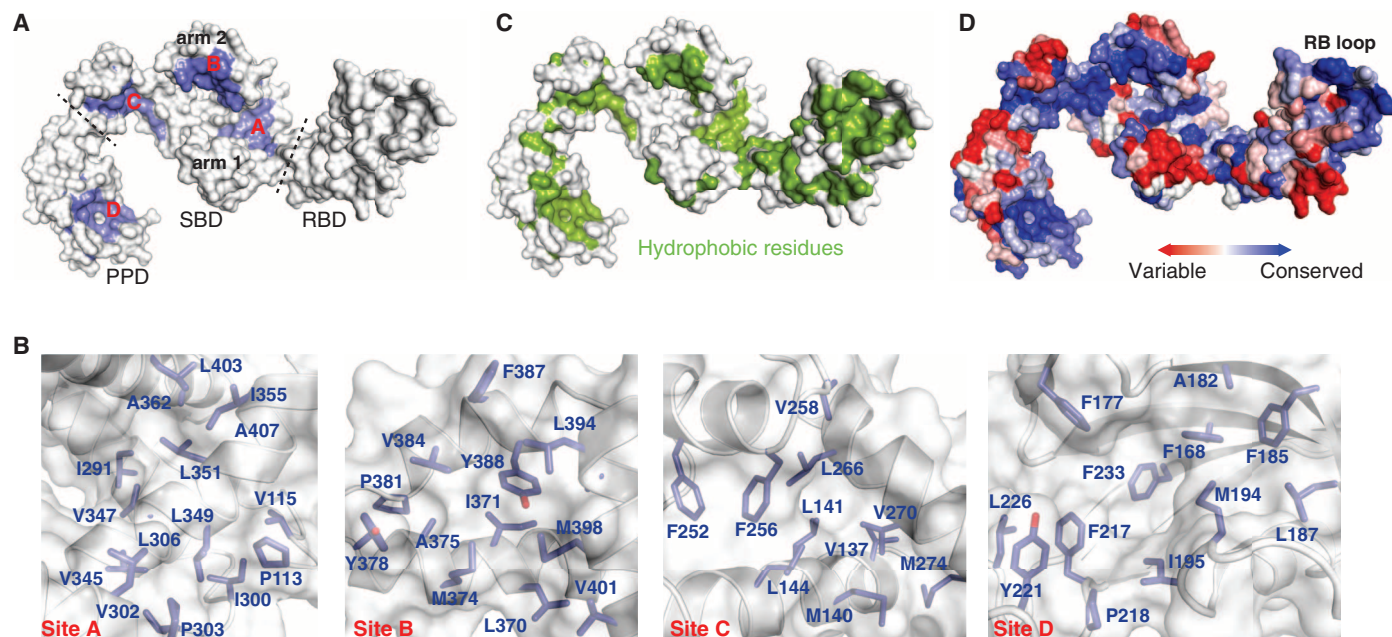
Fig. 1. Substrate-binding sites in TF. (A) The TF residues identified by NMR to interact with unfolded protein substrates are colored blue on the crystal structure of free E. coli TF [Protein Data Bank (PDB) ID 1W26]. The four main binding sites are labeled A, B, C, and D (in red). The dashed lines indicate the domain boundaries. The two structural protrusions in the SBD are labeled arm 1 and arm 2. An additional binding site, located in arm 1, is used by TF to interact with some of the substrates (see Fig. 7A and fig. S11). (B) Expanded
