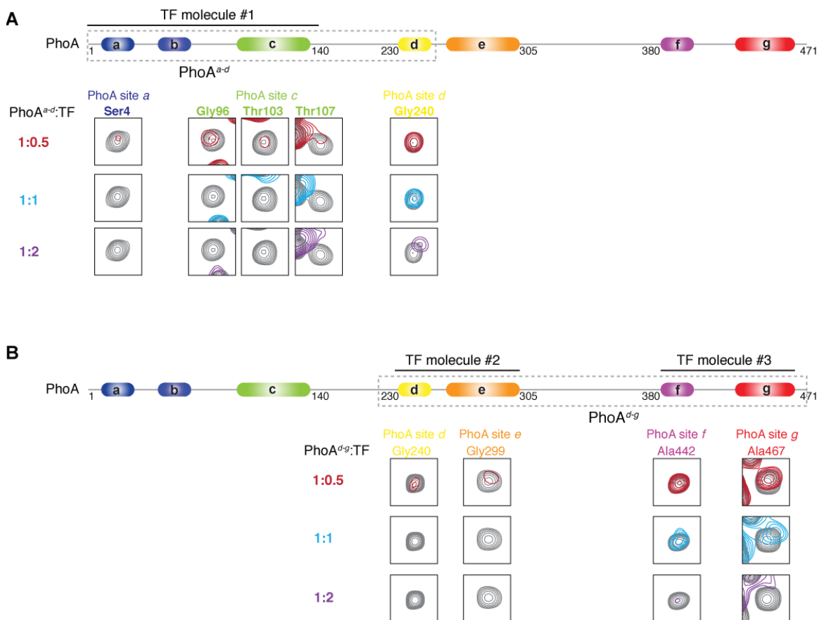
Fig. S16. Synergistic binding and selectivity of PhoA sites for TF. (A) As we explain in detail in Fig. 3, one TF molecule can accommodate sites a and c (residues 1-140). When a longer PhoA fragment that extends to include PhoA site d (PhoA a-d ) is used, then at a stoichiometric ratio of 1:1 (PhoA a-d :TF) site d is not bound by TF. This is clearly demonstrated by the fact that the chemical shift of Gly240 (located in PhoA site d ) is not affected at all. When excess of TF is added (PhoA a-d :TF 1:2) then site d is bound by TF. (B) Direct evidence for synergistic binding among PhoA sites to TF is provided in this experiment. A PhoA fragment consisting of sites d through g was used (PhoA d-g ). Isolated sites d and f bind exclusively to TF PPD (fig. S17B,E) and with very similar affinities (~240 \mu M). One TF molecule binds to PhoA sites d and e , and another TF molecule binds to PhoA sites f and g (Fig. 4A and fig. S17). At substoichiometric PhoA d-g :TF ratio, only PhoA site d , but not PhoA site f , is bound to TF because of the higher affinity of the PhoA d-e fragment, compared to PhoA f-g , for TF (fig. S14). At a PhoA d-g :TF ratio of 1:1, only a small fraction of sites f and g are bound, as dictated by the Boltzmann distribution. Representative peaks from 1 H- 15 N HSQC spectra of labeled TF (TF SBD-PPD ) free (grey) and in complex (red, blue and purple for PhoA:TF ratio 1:0.5, 1:1 and 1:2, respectively) with the corresponding PhoA site are shown. We should note that due to the labeling scheme used for this experiment, and the size of TF, the intensity of the PhoA residues that are bound by TF decreases dramatically or disappears when binding is strong.
