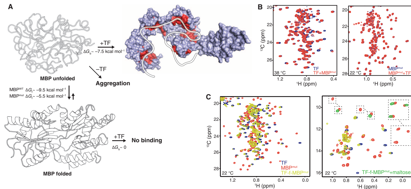
Fig. 7. Antiaggregation and unfoldase activity of TF. (A) Schematic of MBP unfolding and binding reactions between TF and MBP mut . \Delta G_f is the free energy of folding and \Delta G_b is the free energy of binding. The sites that TF uses to interact with the unfolded state of MBP mut , as determined by NMR, are colored red. (B) 1 H- 13 C-correlated methyl NMR spectra of the interaction between TF and MBP mut . The spectrum shown on the left was recorded at 38°C using labeled TF and unlabeled MBP mut , whereas the spectrum shown on the right was recorded at 22°C using the reverse labeling scheme. No interaction was observed at 22°C, where the unfolded population of MBP mut was negligible, whereas binding was observed at 38°C, where the unfolded population of MBP mut was appreciable.
