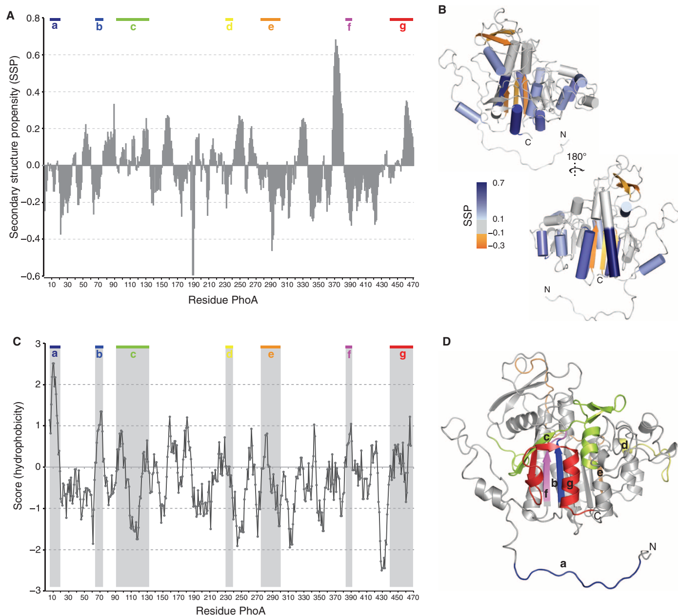
Fig. 2. TF-binding sites and secondary structure in unfolded PhoA. (A) Secondary structure propensity (SSP) values (59) of unfolded PhoA plotted as a function of the amino acid sequence. A SSP score at a given residue of 1 or -1 reflects a fully formed \alpha -helical or \beta -structure (extended), respectively, whereas a score of, for example, 0.5 indicates that 50% of the conformers in the native-state ensemble of the protein are helical at that position. The data show that several of the secondary structure elements in the folded PhoA retain some transient structure in the unfolded PhoA. The TF-binding sites (a to g) are indicated. (B) The SSP values of unfolded PhoA that correspond to secondary
