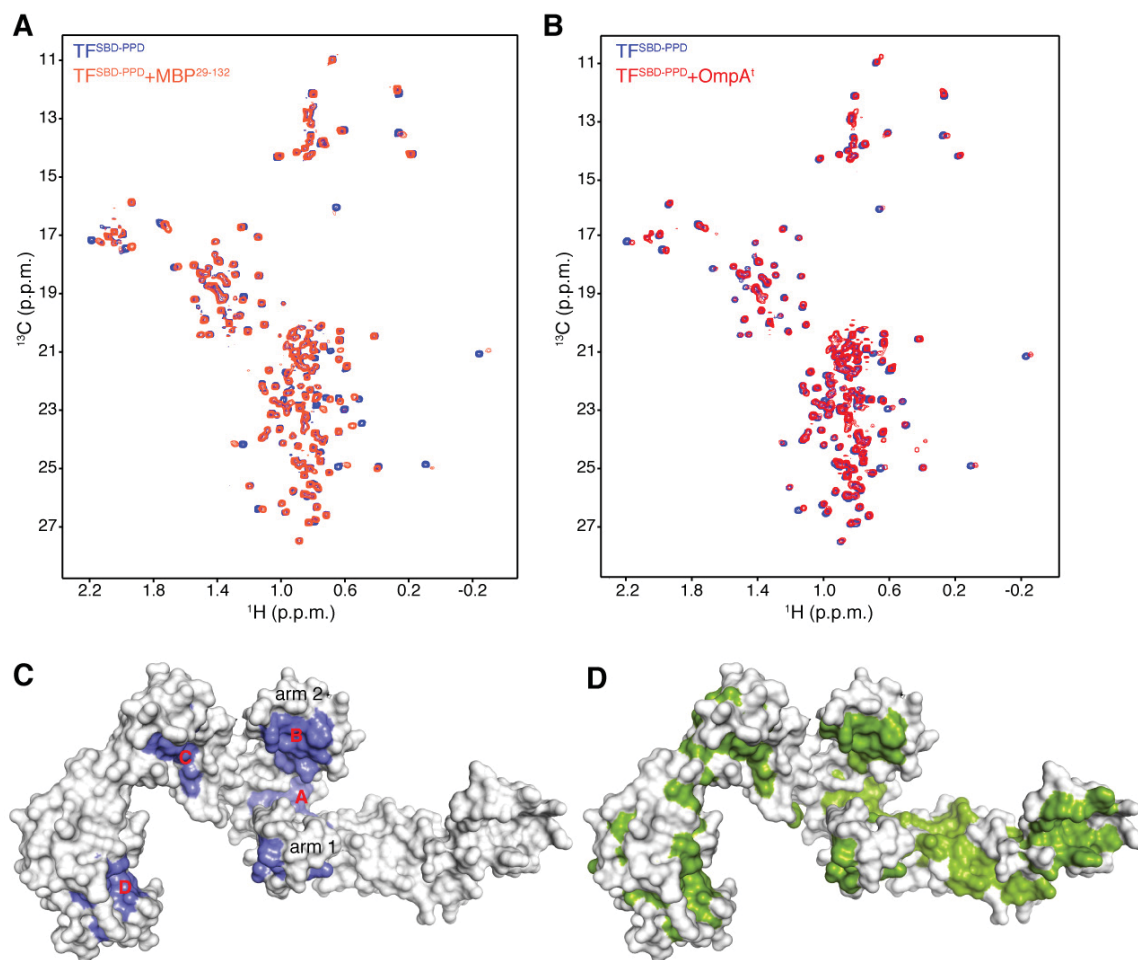
Fig. S11. Interaction of the TF chaperone module (TF SBD-PPD ) with unfolded fragments of the maltose binding protein (MBP) and the transmembrane region of OmpA. (A) ^1\text{H} - ^{13}\text{C} HMQC spectra of [ \text{U} - ^2\text{H} , ^{15}\text{N} ; Ala- ^{13}\text{CH}_3 ; Met- ^{13}\text{CH}_3 ; Ile- \delta 1 - ^{13}\text{CH}_3 ; Leu, Val- ^{13}\text{CH}_3 / ^{13}\text{CH}_3 ]-labeled TF SBD-PPD in complex with a fragment of unlabeled MBP consisting of residues 29-132, which, based on its hydrophobicity (see fig. S26), is predicted to have several TF-binding sites. (B) ^1\text{H} - ^{13}\text{C} HMQC spectra of [ \text{U} - ^2\text{H} , ^{15}\text{N} ; Ala- ^{13}\text{CH}_3 ; Met- ^{13}\text{CH}_3 ; Ile- \delta 1 - ^{13}\text{CH}_3 ; Leu, Val- ^{13}\text{CH}_3 / ^{13}\text{CH}_3 ]-labeled TF SBD-PPD in complex with the transmembrane region of OmpA (OmpA t , residues 1-190). (C) The TF residues identified by NMR (both from backbone and side chain chemical shifts) to interact with MBP 29-132 and OmpA t are colored blue. All four binding sites (A-D) that interact with PhoA also interact with MBP and OmpA. In addition, a hydrophobic region located in arm 1 interacts with MBP and OmpA. As with the other substrate-binding sites, this region is hydrophobic, as can be seen in panel D, which shows the hydrophobic residues in TF (colored green).
