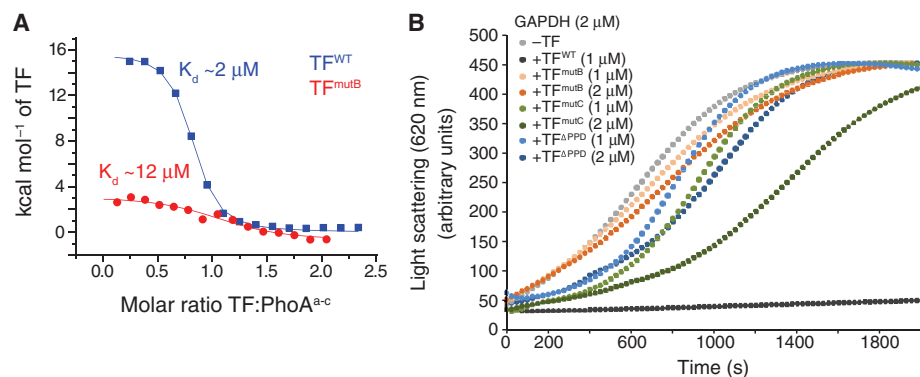
Fig. 5. Effect of mutations in substrate-binding sites on TF activity. (A) Binding affinity determined by ITC for PhoA a-c to TF WT and TF mutB . TF mutB is a mutant in which four hydrophobic amino acids of TF site B were substituted (fig. S23). The mutations result in a sixfold decrease in the affinity. (B) Aggregation of chemically denatured glyceraldehyde-3-phosphate dehydrogenase (GAPDH) monitored by light scattering at 620 nm, in the absence or presence of TF WT and its variants. In contrast to TF WT , TF mutB has very poor antiaggregation activity. The antiaggregation activity is also compromised in TF mutC , a mutant in which a single hydrophobic amino acid of TF site C was substituted (fig. S23), as well as in a TF construct wherein the PPD has been deleted (TF ΔPPD ).
