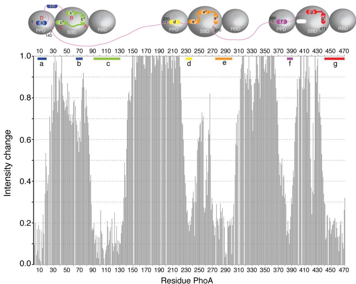
Fig. S15. NMR resonance intensity analysis of the TF-PhoA complex. Plot of resonance intensity changes of PhoA residues as a result of complex formation with TF. Because of the labeling scheme used, PhoA residues that are bound by TF have negligible intensity remaining in the complex, whereas the intensity of residues that are not bound by TF, and are thus motionally not restricted, is not significantly affected. Because of the large size of the TF-PhoA complex, transient interaction of PhoA regions with TF can also result in intensity decrease. The PhoA regions consisting of residues 150-220 and 320-370 do not interact with TF and function as flexible linkers that tether the three PhoA-bound TF molecules.
