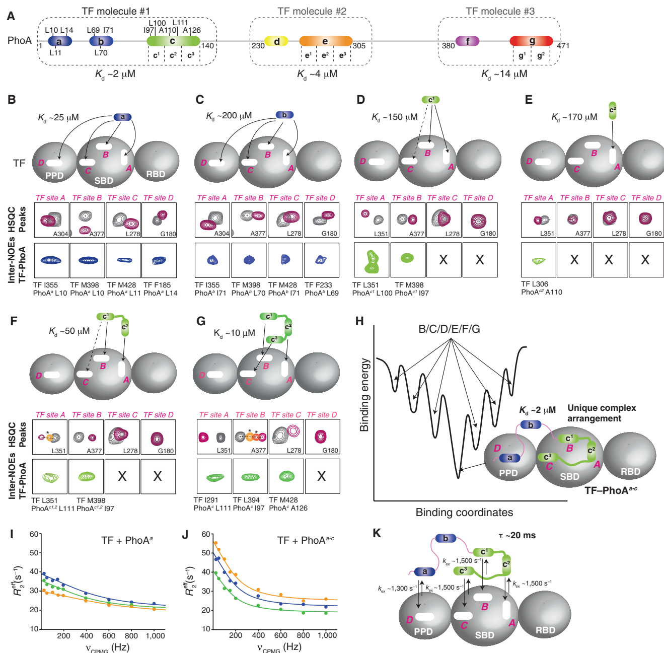
Fig. 3. Dynamic binding and energetics of PhoA by TF. (A) TF-binding sites in PhoA colored as in Fig. 2A. Three TF molecules are required for the simultaneous engagement of the entire PhoA. The K_d for each complex is shown. PhoA residues of sites a, b, and c whose intermolecular NOEs to TF residues are depicted in panels (B) to (G) are indicated. (B to G) The interaction of the independent PhoA site a (B), site b (C), subsite c 1 (D), subsite c 2 (E), subsites c 1 -c 2 (F), and subsites c 1 -c 2 -c 3 (site c) (G) with TF has been characterized by NMR and ITC. The four PhoA-binding sites in TF (A to D) are labeled in pink. In the rectangles labeled “HSQC peaks,” representative peaks from 1 H- 15 N-correlated spectra of labeled TF (TF SBD-PPD ) free (gray) and in complex (magenta) with the indicated PhoA site are shown. In the rectangles labeled “Inter-NOEs TF-PhoA,” representative intermolecular NOEs between the TF and PhoA residues are shown. The full NOESY strips are shown in fig. S13. The symbol X indicates the absence of such NOEs. The K_d values were determined by ITC and NMR. Solid arrows indicate experimentally observed binding of the PhoA site to the designated TF site. Broken arrows indicate transient interaction observed by chemical shift perturbation but for which no intermolecular NOEs were detected. The orange cross peak (marked with an asterisk) for TF site A in panel (F) corresponds to the chemical shift observed for the binding of the individual subsite c 2 to TF site A shown in panel (E). Similarly, the orange and dark-orange cross peaks
