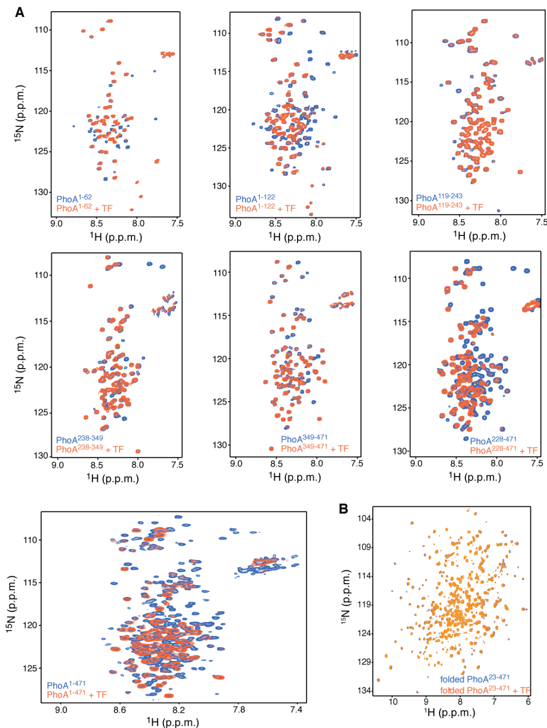
Fig. S7. Identification of the TF-binding sites in PhoA by NMR. (A) ^{15}\text{N} labeled full-length PhoA as well as a number of PhoA fragments were titrated with unlabeled TF. Due to the labeling scheme and the size of TF, the intensity of the PhoA residues that are bound by TF decreases dramatically or disappears. The ^1\text{H} - ^{15}\text{N} HSQC spectra of PhoA select fragments and the full-length PhoA are shown in the absence (blue) and presence (orange) of TF. The fragments cover the entire sequence of PhoA and the regions identified to interact with TF in the various PhoA fragments are essentially identical to the full-length PhoA. (B) Oxidized, folded PhoA (mature form) does not interact with TF.
