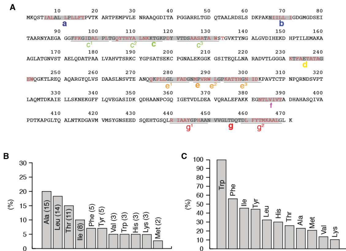
Fig. S8. Amino acid composition of TF-binding sites in PhoA. (A) Primary sequence of PhoA with the TF-binding sites (a-g) highlighted. The PhoA residues that form direct contacts with TF are colored red (see Fig. 4). The color code of the sites and subsites are as in Fig. 2C and 3A. (B) Percentage values of the PhoA amino acids that directly interact with TF. The number in brackets correspond to the actual number of amino acids. (C) Percentage values of PhoA amino acids that interact with TF normalized against the total number of each one of the amino acids in the PhoA sequence. For example, all of the three Trp residues in PhoA interact with TF (that is, 100%).
