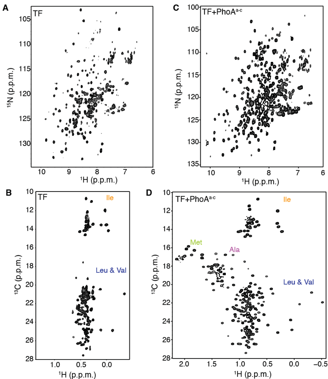
Fig. S2. NMR spectra of unliganded TF and in complex with PhoA. (A) ^1\text{H} - ^{15}\text{N} TROSY HSQC of [\text{U-}^2\text{H}, ^{15}\text{N}] -labeled and (B) ^1\text{H} - ^{13}\text{C} methyl HMQC spectra of [\text{U-}^2\text{H}; \text{Ile-}\delta 1\text{-}^{13}\text{CH}_3; \text{Leu, Val-}^{13}\text{CH}_3/^{13}\text{CH}_3] -labeled dimeric TF (unliganded). Analysis of the spectra shows that several resonances are broadened beyond detection, presumably because of slow motions at the dimeric interface (see fig. S19). (C) ^1\text{H} - ^{15}\text{N} TROSY HSQC of [\text{U-}^2\text{H}, ^{15}\text{N}] -labeled and (D) ^1\text{H} - ^{13}\text{C} methyl HMQC spectra of [\text{U-}^2\text{H}; \text{Ala-}^{13}\text{CH}_3; \text{Met-}^{13}\text{CH}_3; \text{Ile-}\delta 1\text{-}^{13}\text{CH}_3; \text{Leu, Val-}^{13}\text{CH}_3/^{13}\text{CH}_3] -labeled TF in complex with PhoA a-c . Analysis of the spectra indicates that all of the expected resonances are present. The dispersion and sensitivity of these spectra are excellent. Both TF and PhoA a-c are labeled.
