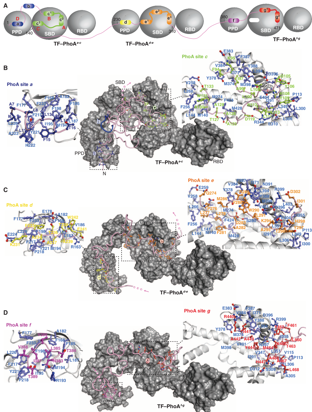
Fig. 4. Structural basis for the formation of the TF-PhoA complexes. (A) Schematic for the interaction of PhoA with TF based on the current structural data. The TF-binding sites in PhoA are colored as in Figs. 2 and 3A. (B to D) Lowest-energy structure of the three TF molecules in complex with the corresponding PhoA regions. TF is shown as a solvent-exposed surface and PhoA as a pink ribbon. The PhoA residues that directly interact with TF are drawn in a ball-and-stick representation, colored as in panel (A). The pink arrows denote the
