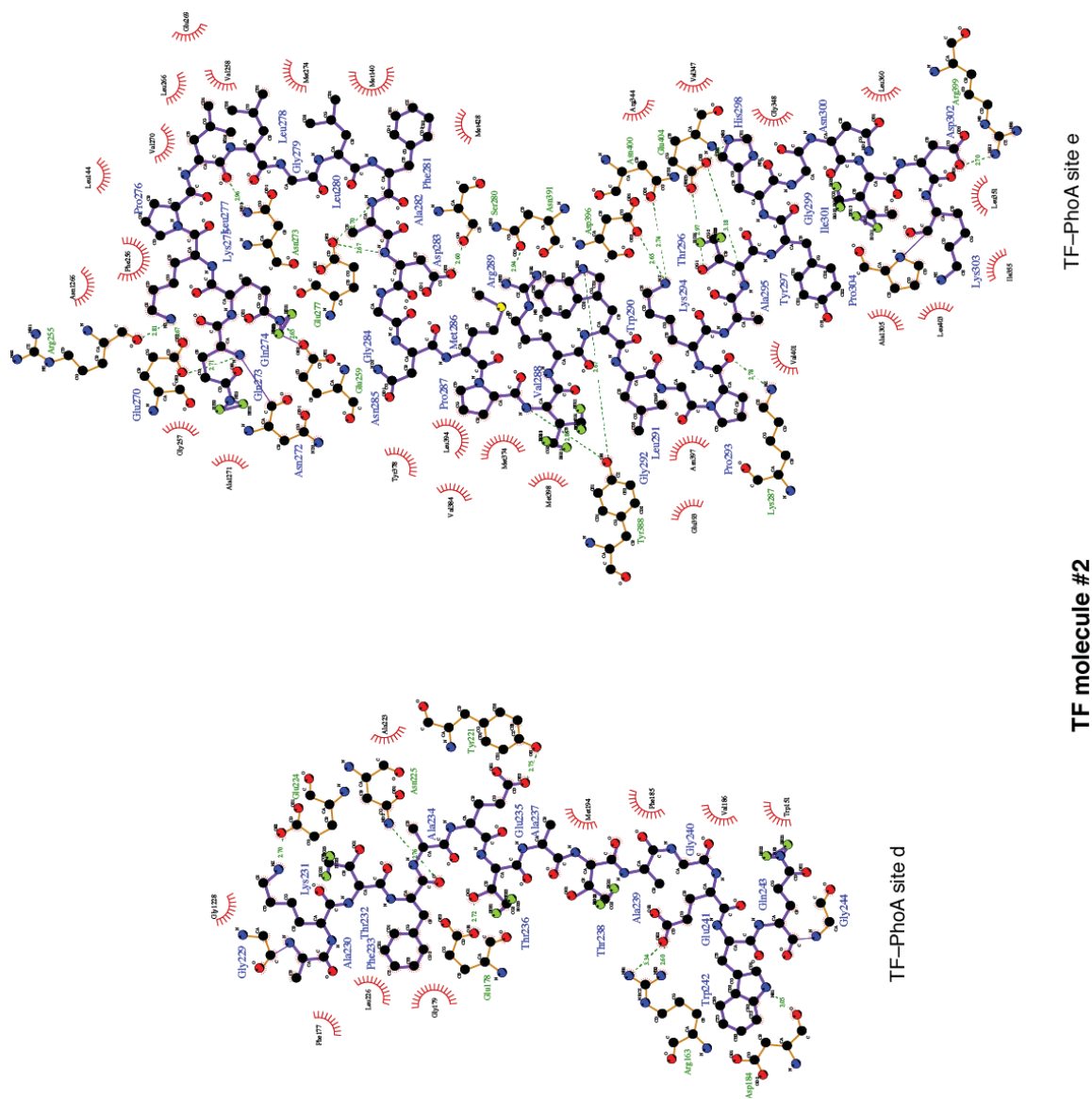
Fig. S21. TF-PhoA d-e contacts. Inter-molecular contacts between TF and PhoA d-e generated by Ligplot.
