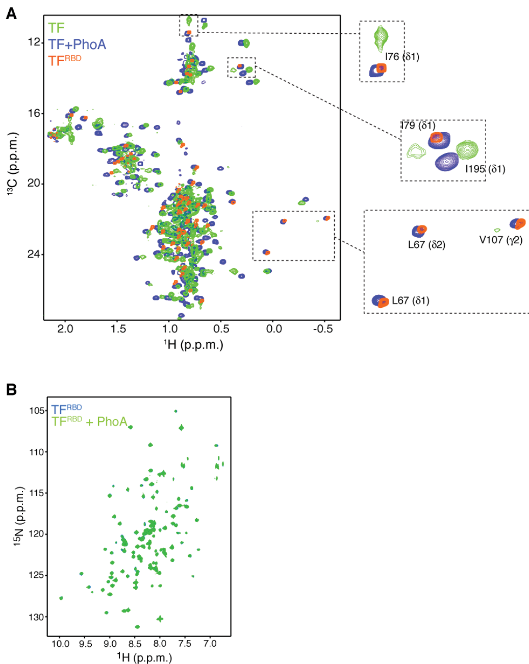
Fig. S18. PhoA binding monomerizes TF. (A) ^1\text{H} - ^{15}\text{N} HSQC spectra of TF (green), in complex with unlabeled PhoA (blue), and isolated RBD (orange). TF and TF RBD are [U- ^2\text{H} , ^{15}\text{N} ; Ala- ^{13}\text{CH}_3 ; Met- ^{13}\text{CH}_3 ; Ile- \delta 1 - ^{13}\text{CH}_3 ; Leu, Val- ^{13}\text{CH}_3 / ^{13}\text{CH}_3 ] labeled. Analysis of the spectra shows that several resonances in free TF, which is dimeric (fig. S1C), are broadened beyond detection, presumably because of slow motions at the dimeric interface (fig. S19). NMR analysis demonstrates that TF dimerization is mediated by all three domains (RBD, SBD, and PPD) but RBD resonances in TF are particularly affected (fig. S19). Indeed, monomerization of TF upon PhoA binding (fig. S1C-E) results in the appearance of all of the expected resonances (see for example residues L67, I76, I79 and V107). Furthermore, chemical shift comparison between isolated RBD (orange) and TF in complex with PhoA (blue) suggests that RBD does not bind to PhoA. (B) This observation is further corroborated by NMR titration data of ^{15}\text{N} labeled RBD with PhoA (green). The ^1\text{H} - ^{15}\text{N} HSQC spectra show no perturbation.
