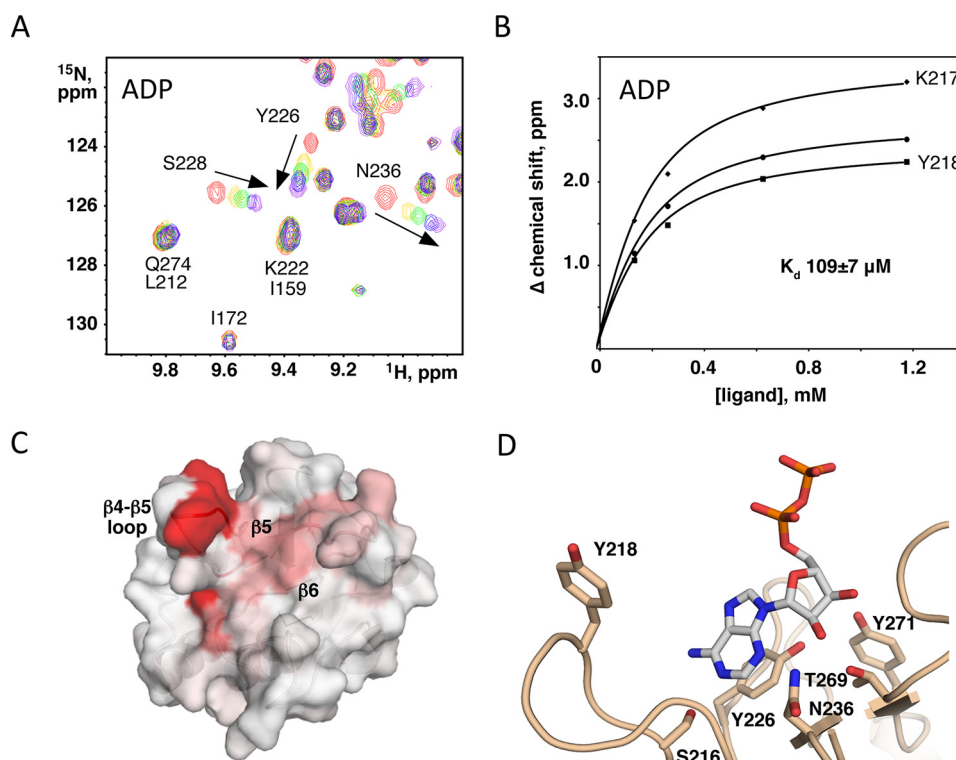
FIGURE 4. KLAMP2 ADP binding. A , downfield region of HSQC spectra of 15 N-labeled KLAMP2 domain titrated with increasing amounts of ADP at 0 mM (red), 0.13 mM (yellow), 0.26 mM (green), 0.63 mM (blue), and 1.18 mM (purple). The spectra show specific chemical shift changes for a number of signals. B , K d of the binding estimated from a fit of the 15 N chemical shift changes for two assigned and one unassigned signal that show large chemical shift changes. C , mapping of the chemical shifts measured onto the structure of the KLAMP2 domain. Red indicates largest chemical shift changes; white indicates no change detected. The most affected surface is centered on the β4–β5 loop and strands β5 and β6. D , model of an ADP-bound KLAMP2 domain based on the 3',5'-cAMP/KLAMP1 structure, with residues important for binding shown.
