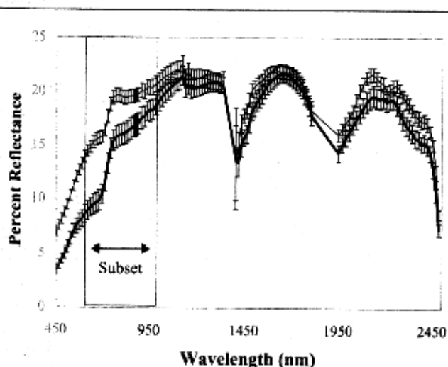
Figure 2. Spectral profiles derived from burned (upper spectra, 22 sample mean) and unburned (lower spectra, 18 sample mean) areas. Typical burned areas lack any sagebrush, while the unburned areas had relatively high percent sagebrush cover. The spectral range used for the final hyperspectral analysis is noted.
