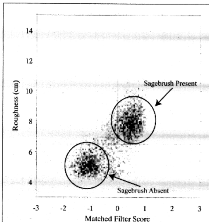
Figure 4. Scatterplot of Matched Filter (MF) score versus surface roughness for the entire study area, illustrating the relationship between areas of sagebrush presence (higher MF and higher roughness) and sagebrush absence (lower MF and lower roughness). Lines represent the roughness threshold of 6.5 cm and the MF threshold of zero that were used to generate sagebrush classifications.
