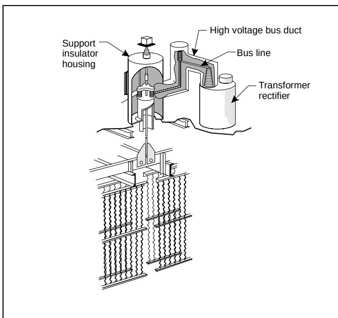
Figure 2-10. High-voltage system
