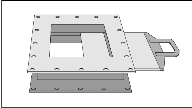
Figure 2-16. Slide-gate
