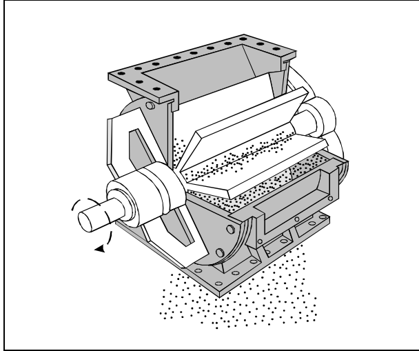
Figure 2-18. Rotary airlock discharge device
