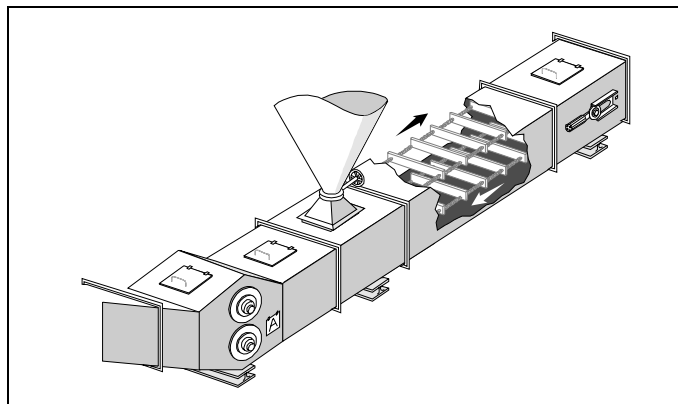
Figure 2-20. Drag conveyor
