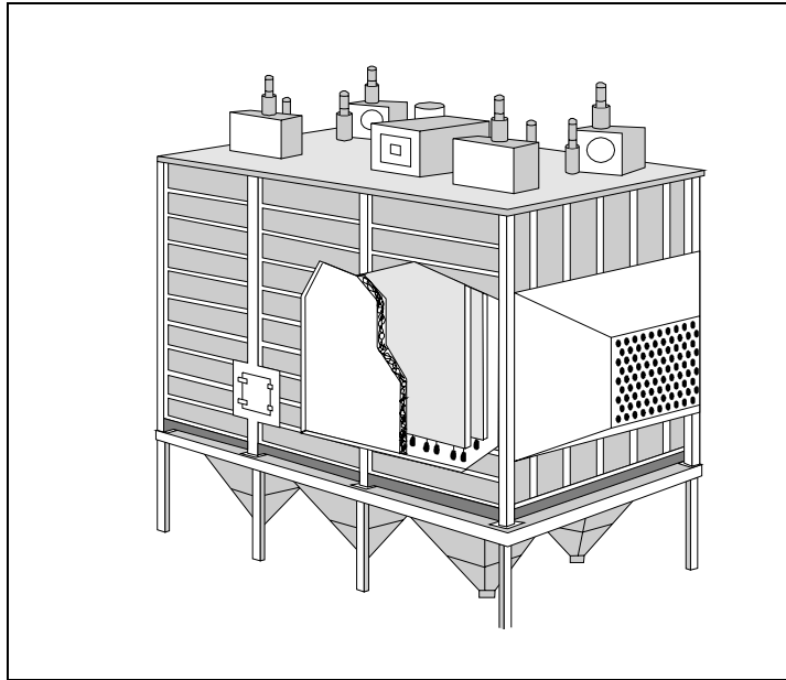
Figure 2-22. ESP shell
