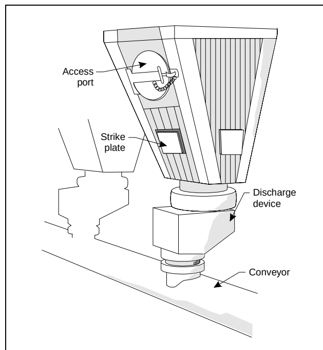
Figure 2-15. Hopper
