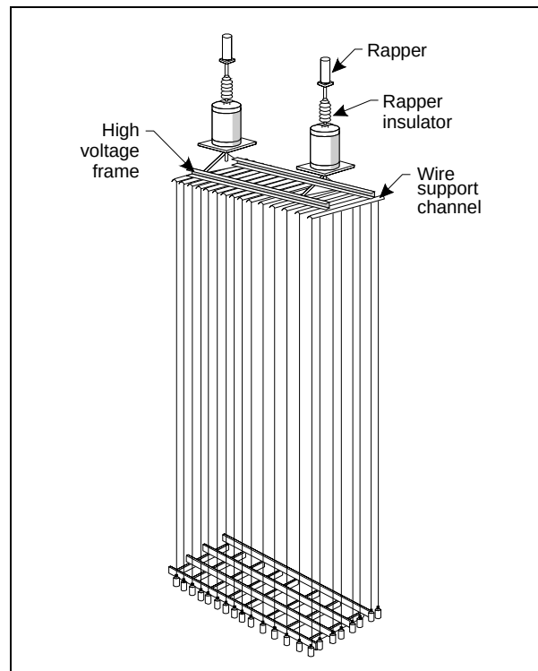
Figure 2-14. Typical electric-vibrator rappers used for wire discharge electrodes
