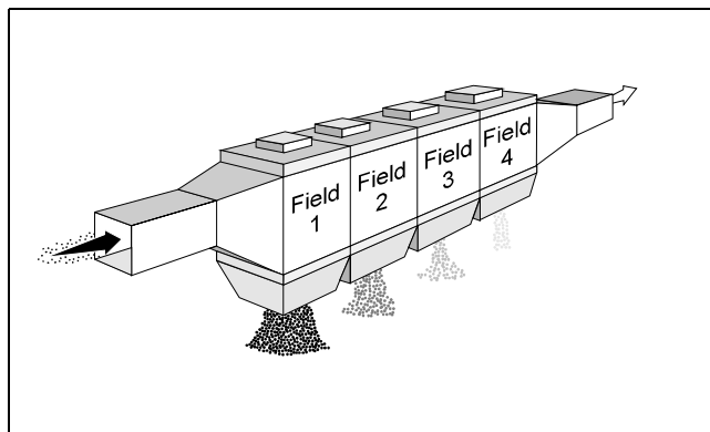
Figure 3-5. Field sectionalization
