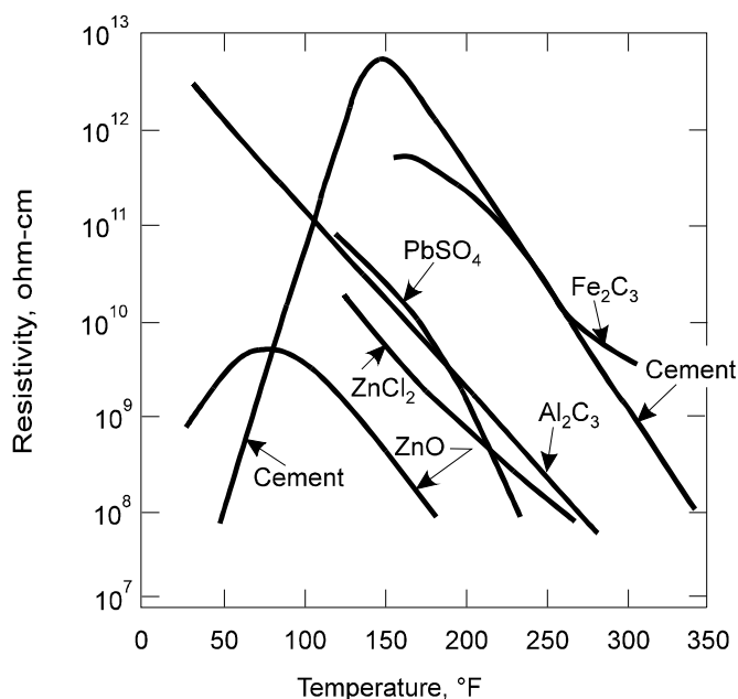
Figure 3-1. Resistivity of six different dusts at various temperatures Source: U.S. EPA 1985.
