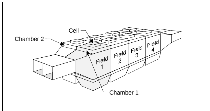
Figure 3-6. Parallel sectionalization (with two parallel sections, eight cells, and four fields)
