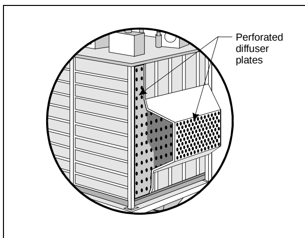
Figure 3-7. Gas inlet with perforated diffuser plates
