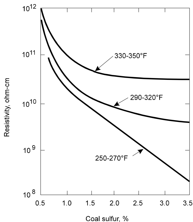
Figure 3-3. Fly ash resistivity versus coal sulfur content for several flue gas temperature bands Source: White 1977.
