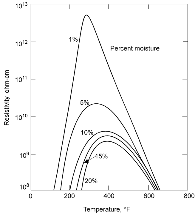
Figure 3-2. Effect of temperature and moisture on the resistivity of cement dust
