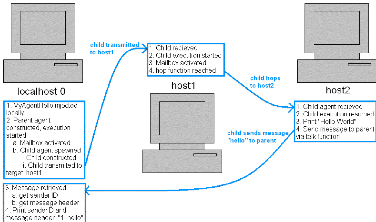
Figure 5: Talk is used to pass a message from a child agent to a parent.
