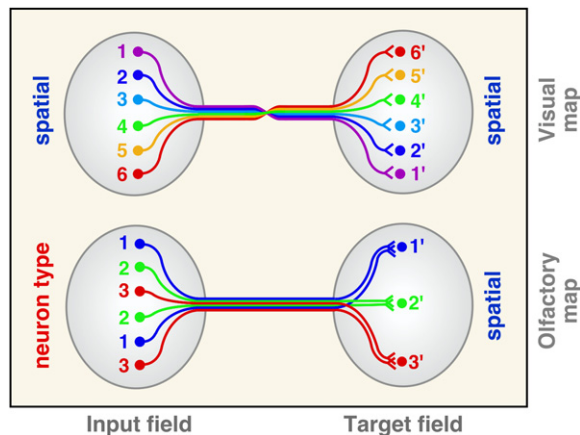
Figure 1. Continuous and Discrete Neural Maps
