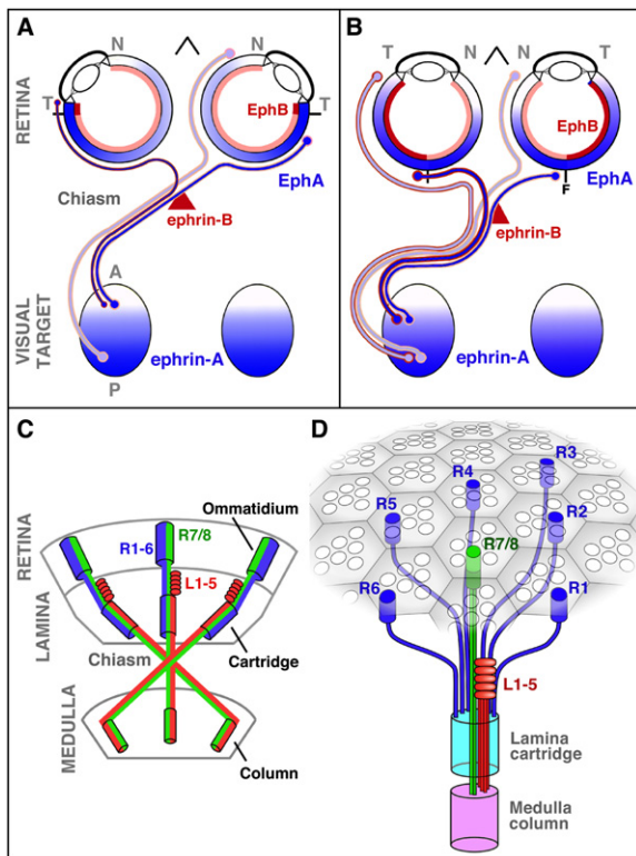
Figure 2. Topographic Organization of Retinal Projections
