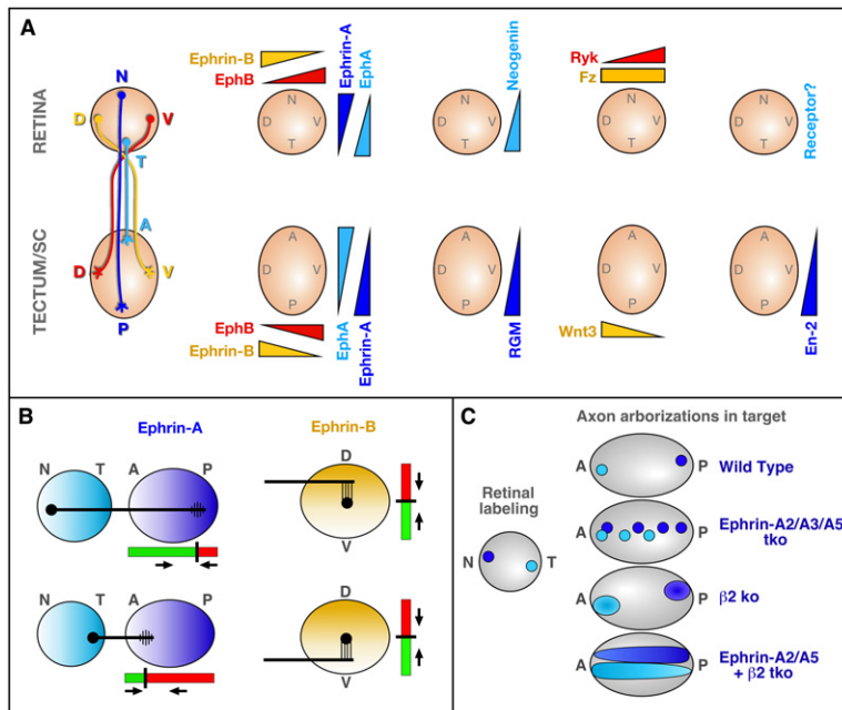
Figure 3. Gradients, Bifunctional Guidance Mechanisms, and Neural Activity in the Retinotectal Projection
