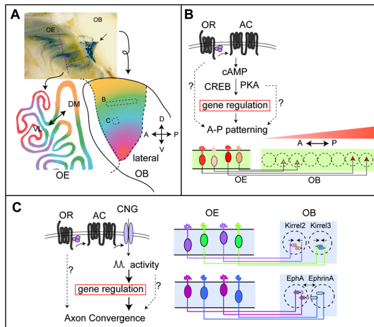
Figure 4. Organization and Development of the Mouse Olfactory Map
