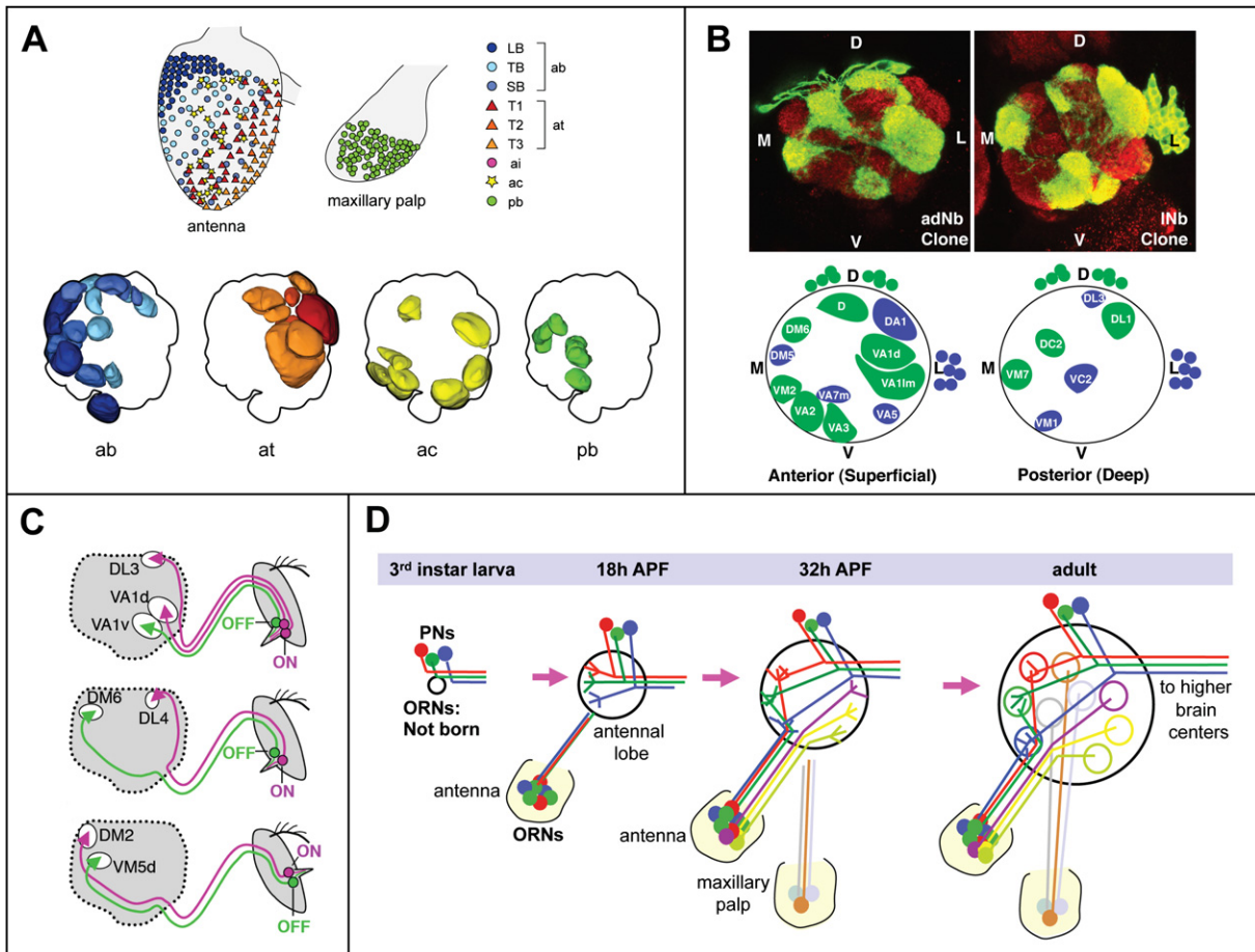
Figure 5. Organization and Development of the Fly Olfactory Map
