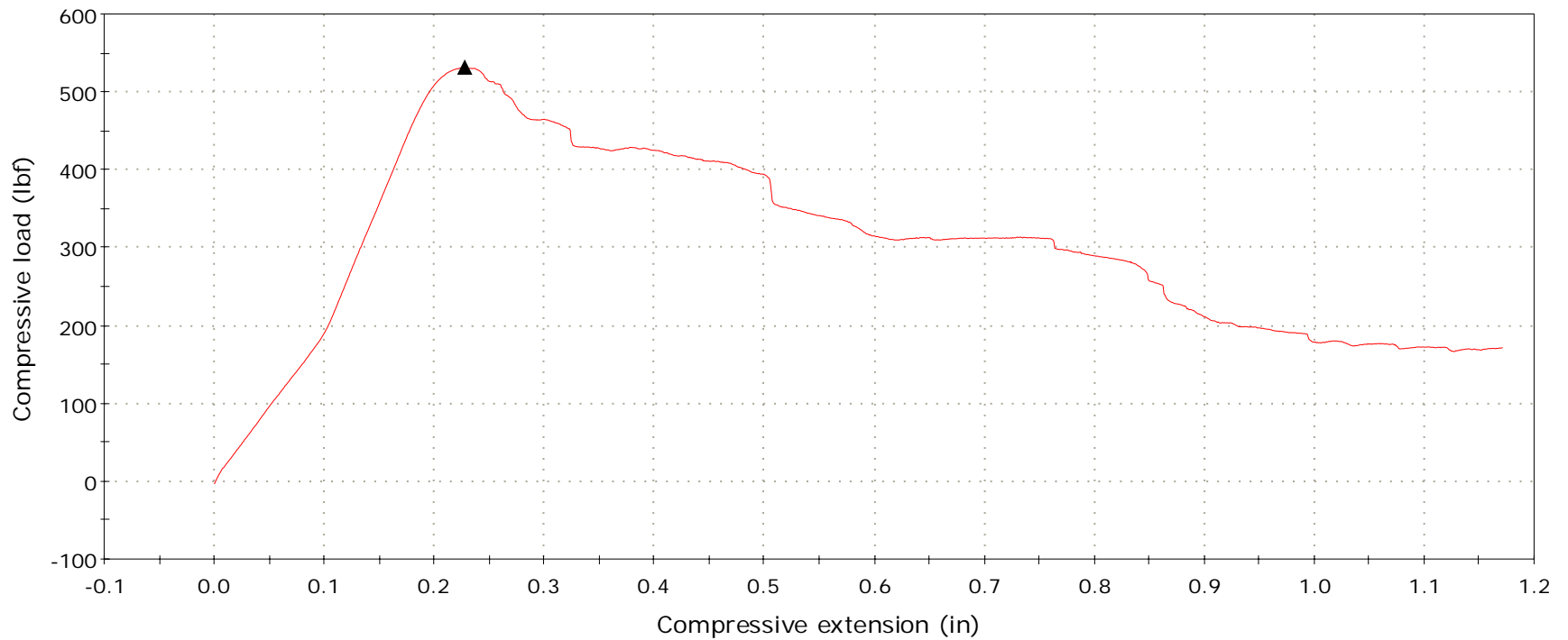
Load vs. Extension
