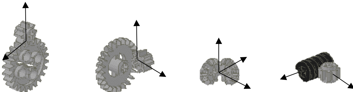
Figure 2-32. Forces on gears
