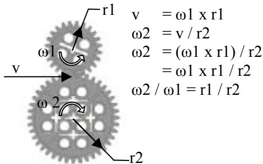
Figure 2-11. Ratio of Angular Velocities is Equal to Inverse Ratio of the Radii
