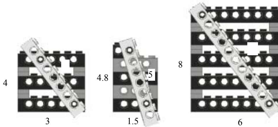
Figure 1-18. Diagonal Cross Bracing
