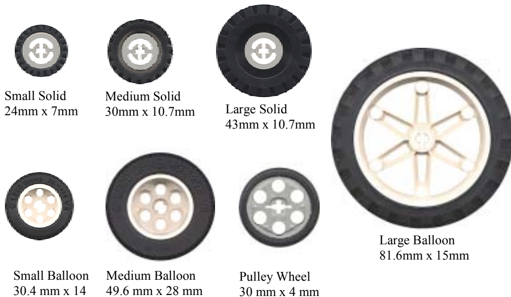
Figure 3-1. Lego Wheels and Tires
