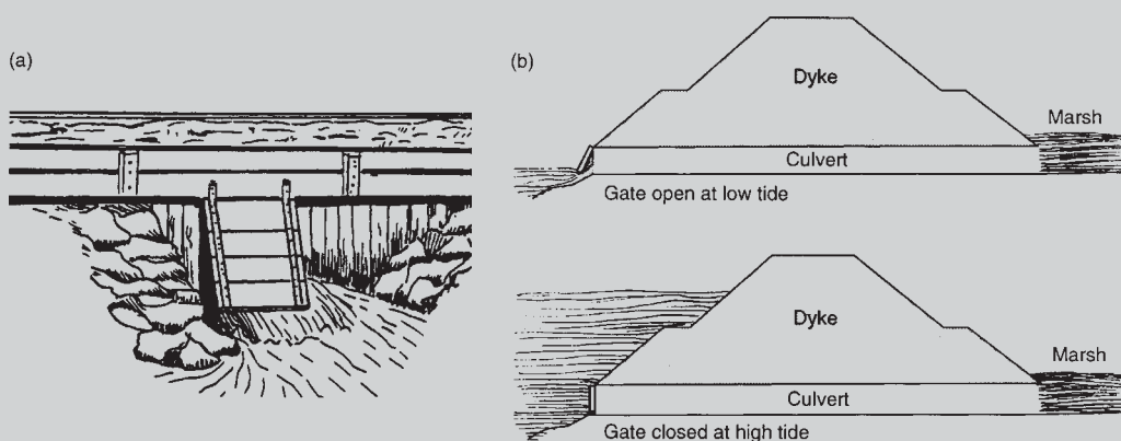
Fig. 1.130 Sluice gates can allow swamps to drain into the sea, while preventing influx of seawater at high tide (133).
