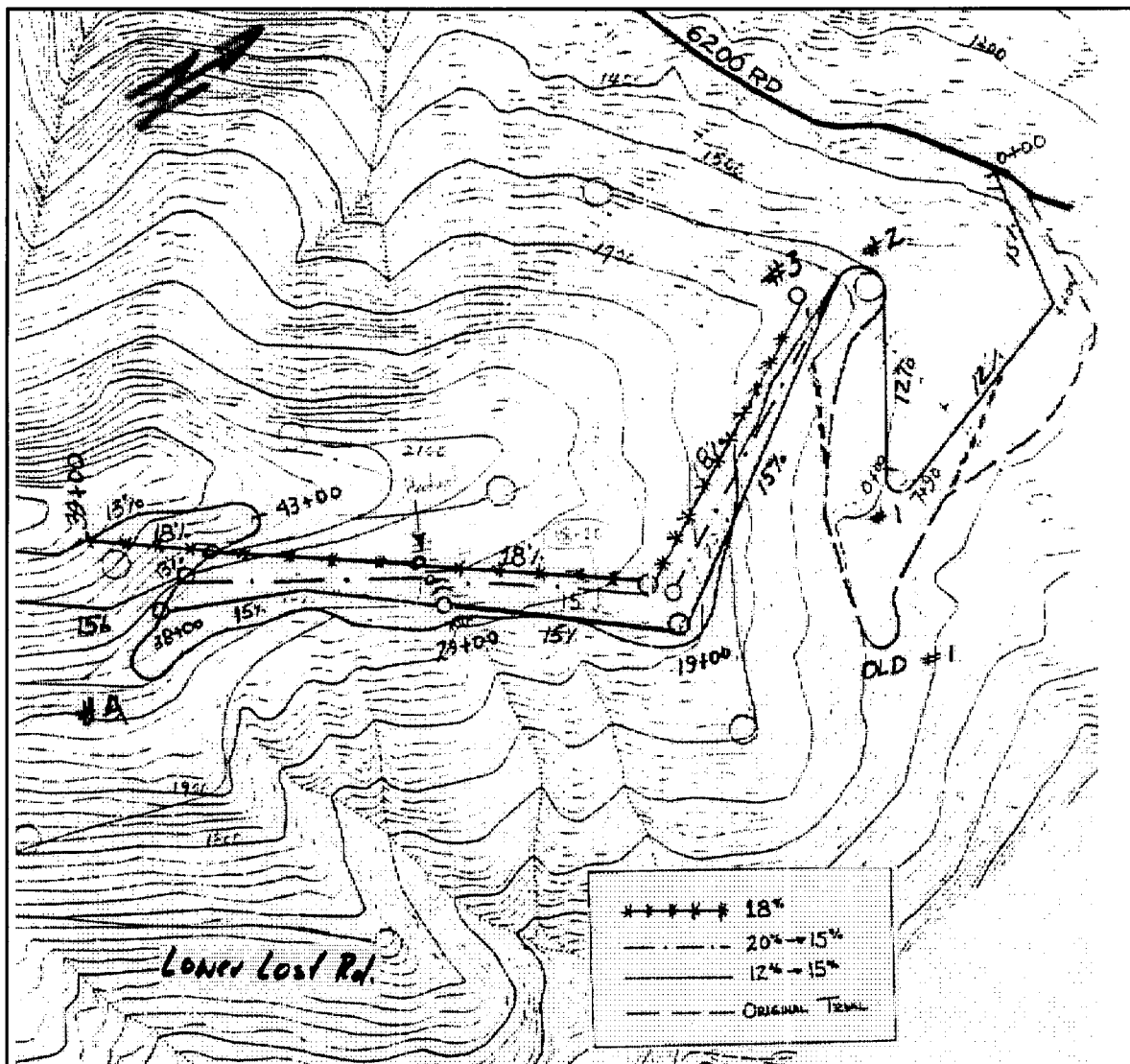
Fig 4.2.3: Lost Road lower grade line trials showing switchback locations
