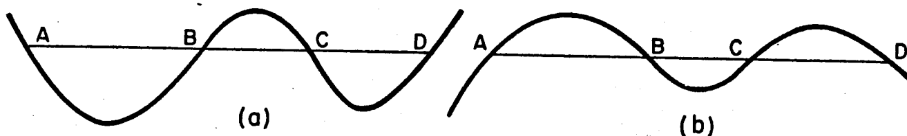
Fig. 4— Mass curves with three loops.
