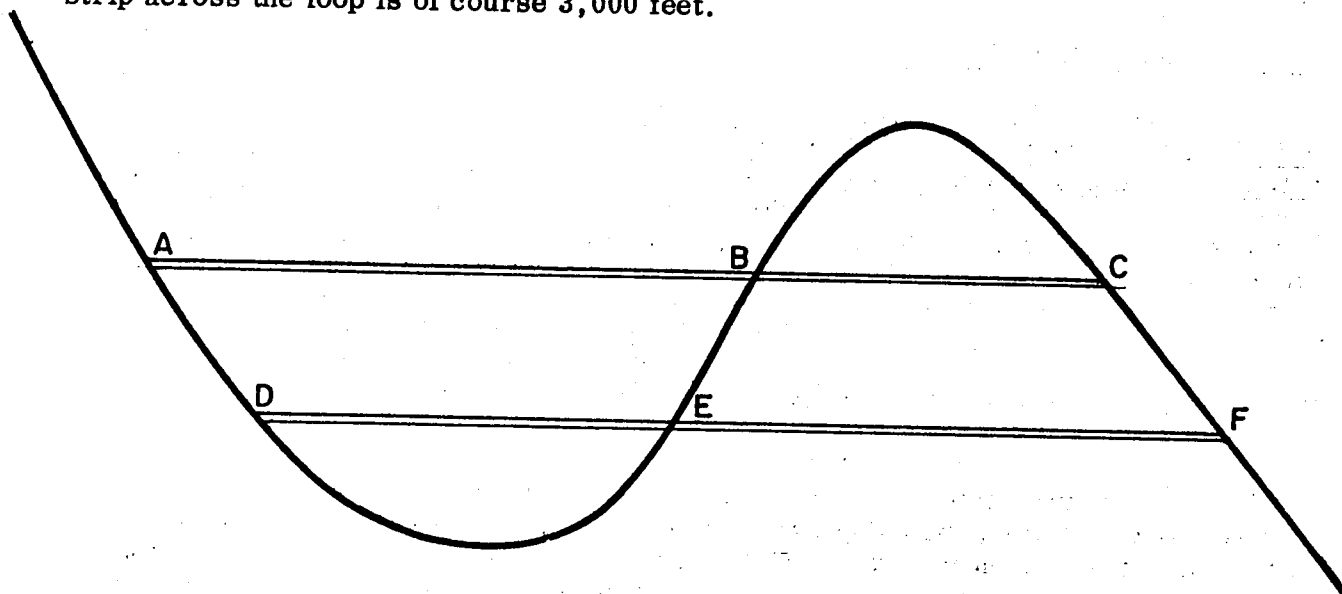
Fig. 7— Mass curve with pair of loops.
