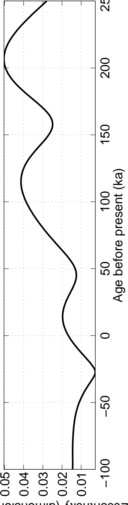
Eccentricity (dimensionless)
