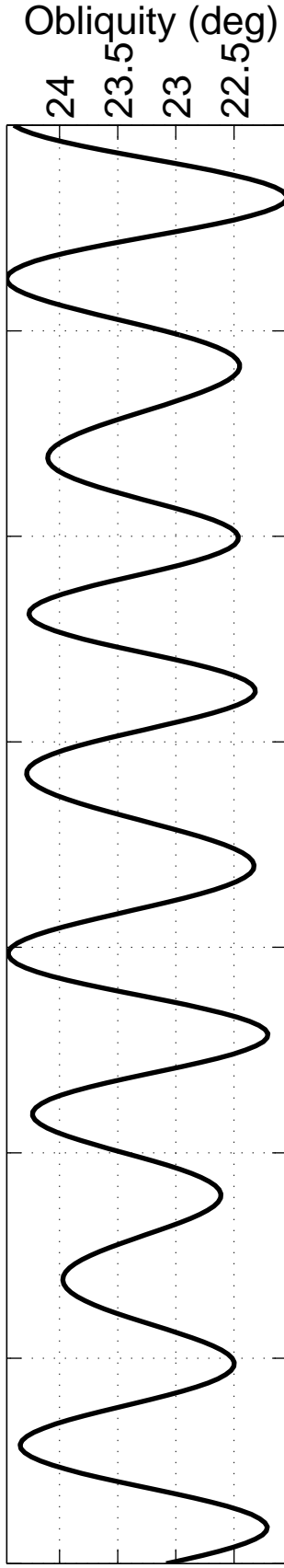
Obliquity
