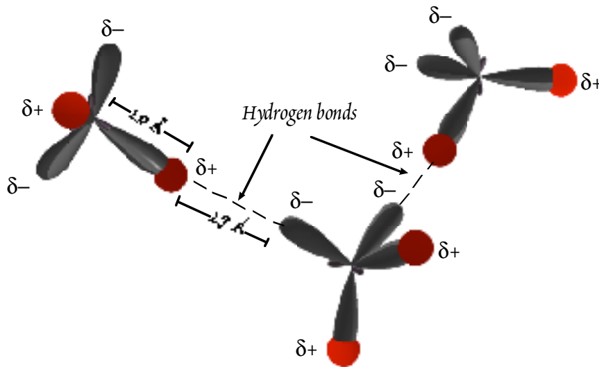
Figure 1.8. Hydrogen bonding between water molecules. Hydrogen positions shown as red; sp 3 hybrid orbitals in oxygen shown as dark gray. The \delta+ and \delta- indicate partial positive and negative charges respectively.
