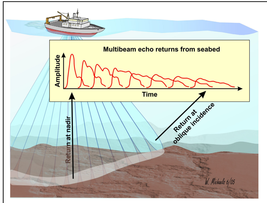
Figure 7.12. Generalized diagram showing changes in multibeam echo returns from the seabed in relation to the angles of incidence within the swathe.
