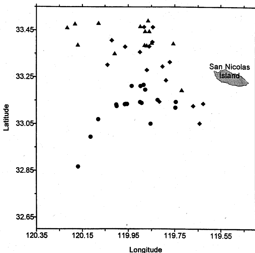
Fig. 5. Location of orqual sightings during pre-experimental (circles), experimental (diamonds) and post-experimental (triangles) periods of exposure to human-produced LFS in the vicinity of San Nicolas Island, California.
