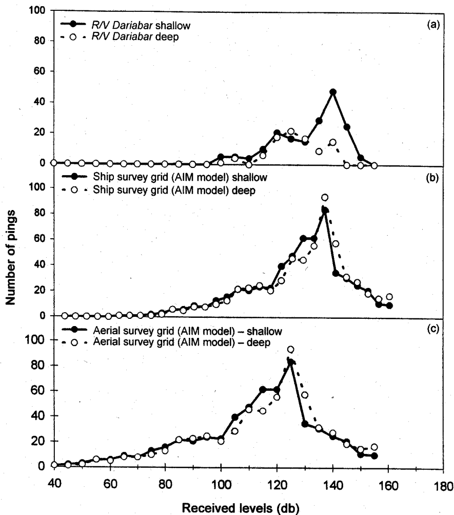
Fig. 2. Levels of anthropogenic LF noise (a) received by R/V Dariabar (ship-based) in San Nicolas Island, California study area, (b) estimated for the ship-based survey area using an acoustic integration model (AIM), and (c) estimated for the aerial-based survey area using an acoustic integration model (AIM). The shallow hydrophone was towed at 10 m, the deep hydrophone was towed at 83 m. The acoustic integration model (AIM) was run for shallow (50 m) and deep (200 m) depths
