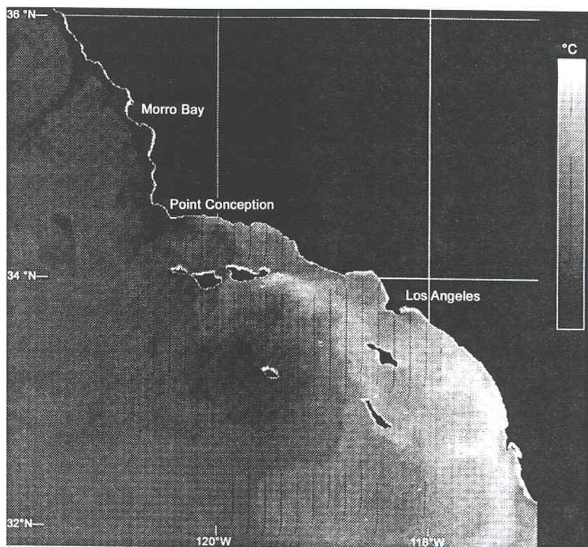
Fig. 7. Sea Surface Temperature (SST) recorded by the NOAA AVHRR satellite in the Southern California Bight, California region on September 10, 1997. San Nicolas Island (white arrow) is located in upwelling plume, indicated by colder water, south of Pt. Conception.
