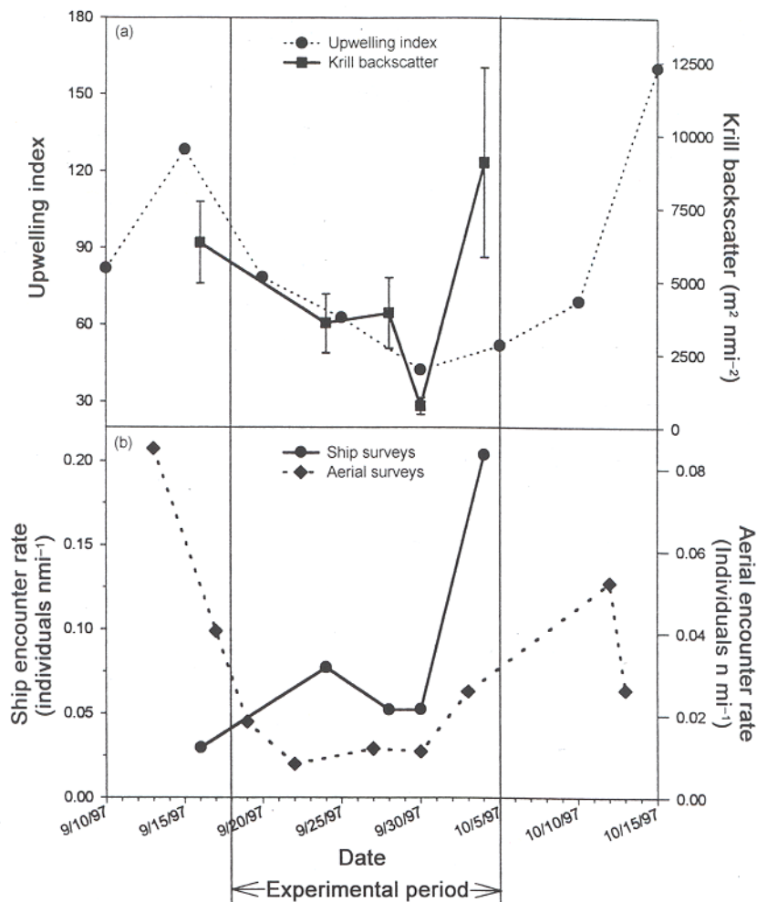
Fig. 3. (a) Bakun upwelling index (dotted line) and krill backscatter (continuous line), (b) whale encounter rate in ship surveys (continuous line) and whale encounter rate in aerial surveys (dotted line) measured before, during, and after exposure to human-produced LFS in the vicinity of San Nicolas Island, California.
