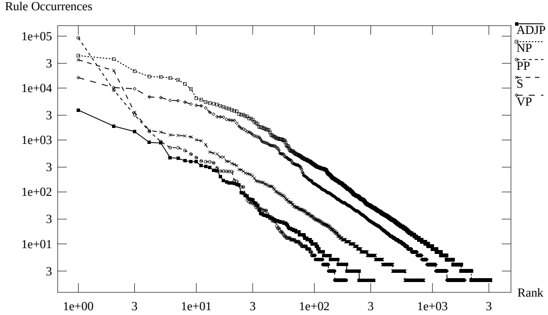
Figure 2: Distribution of Rule Occurrences by Rank
