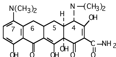
Minocycline
