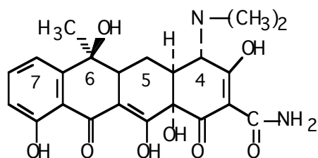
Tetracycline
