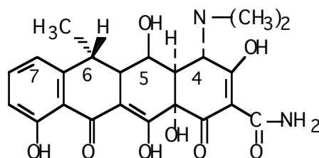
Doxycycline
