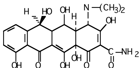
Oxytetracycline
