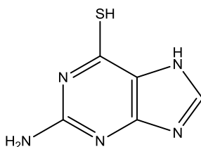
Thioguanine
