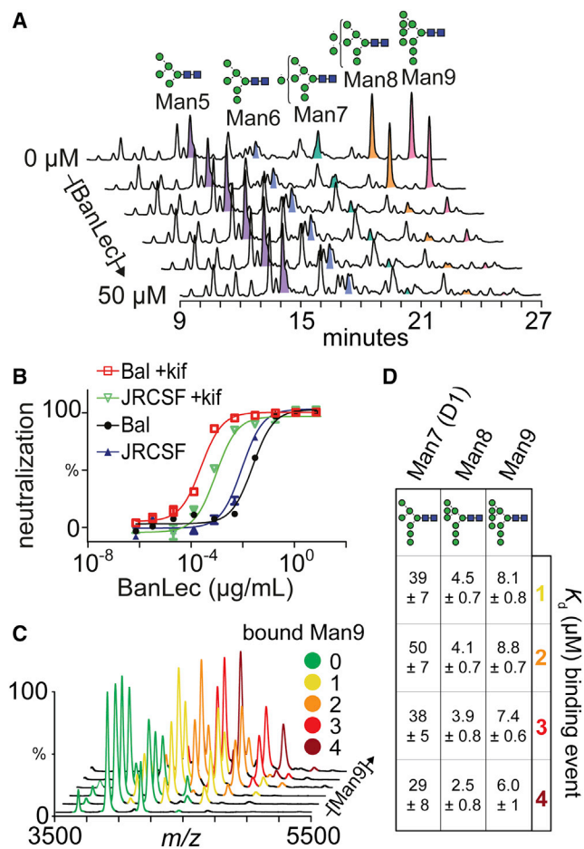
Figure 1. N-Glycan-Binding Assays to BanLec and Inhibition Assays (A) HPLC depletion assay of released gp120 N-glycans incubated with 0, 1, 5, 10, 20, and 50 \mu\text{M} BanLec. (B) Inhibition of HIV pseudovirus strains JRCSF and BaL expressed with and without kifunensine (kif). (C) Native mass spectra of BanLec with different concentrations of Man9 (0, 2.5, 7.5, 15, 30, and 50 \mu\text{M} ). (D) K_d s determined from MS experiments binding Man7, Man8, and Man9 to BanLec, and calculated from peak intensities.
