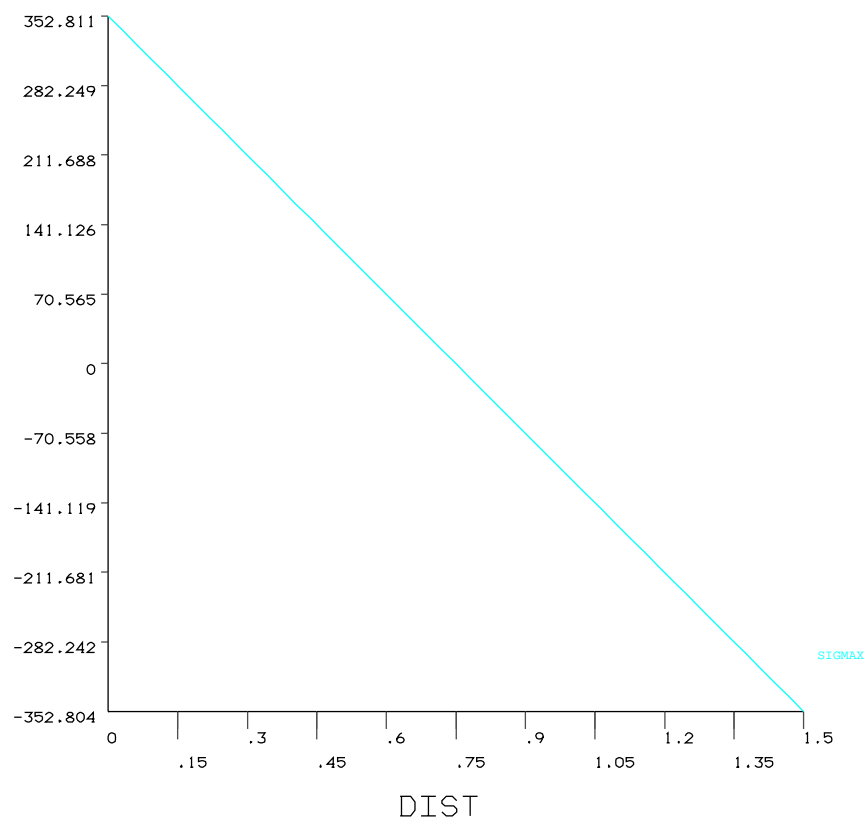
Notched Beam
