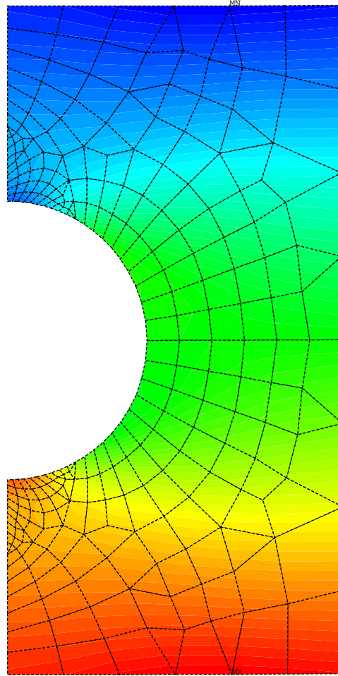
Stress concentration for beam with central hole
