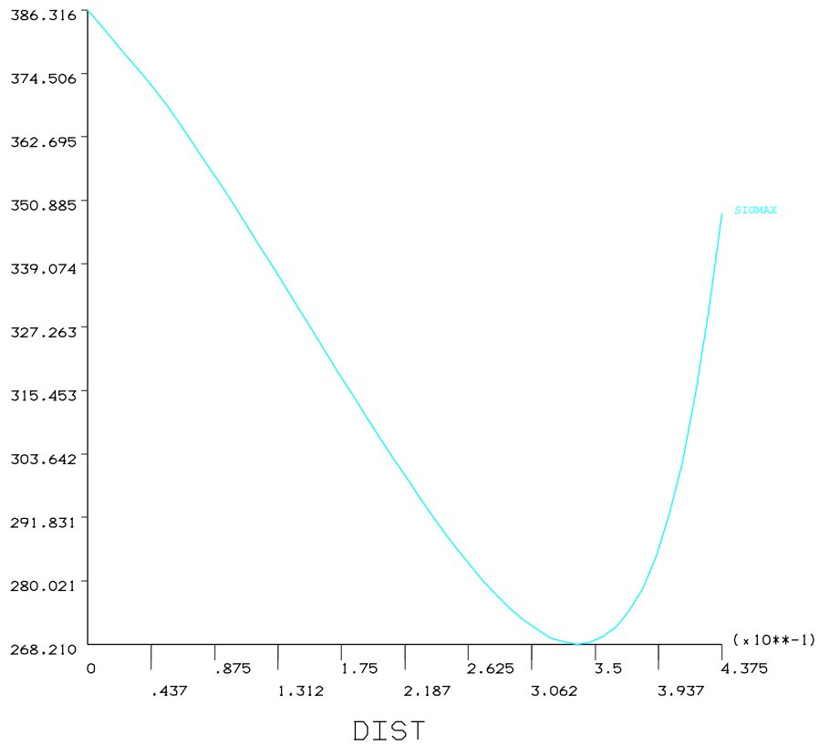
Stress concentration for beam with central hole
