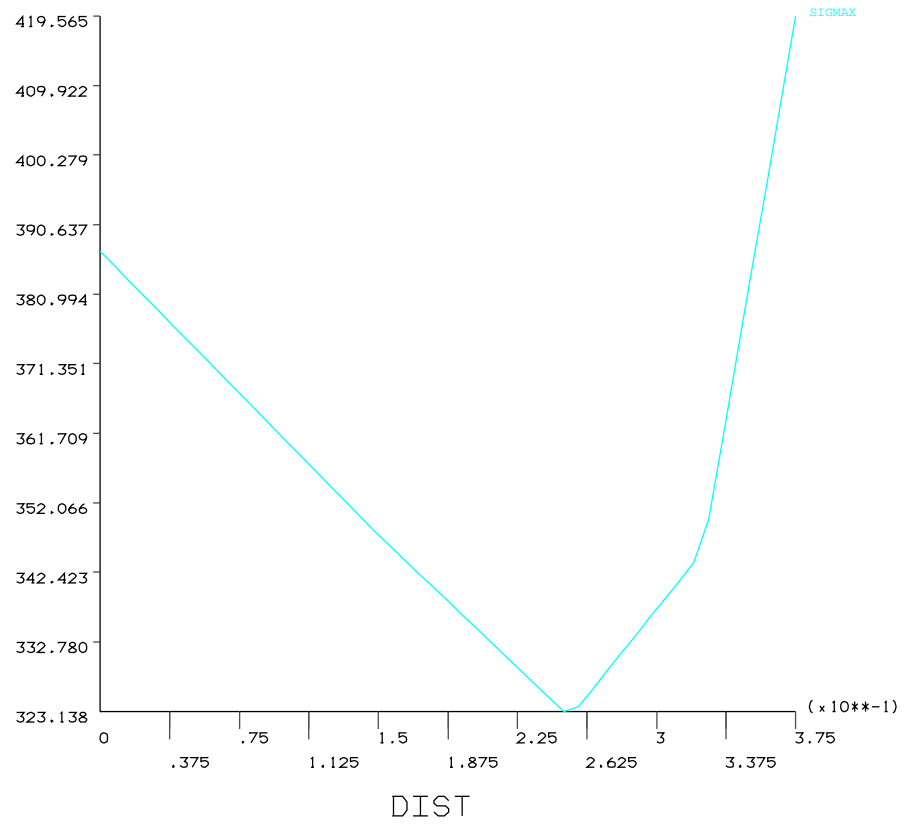
Stress concentration for beam with 2 central holes
