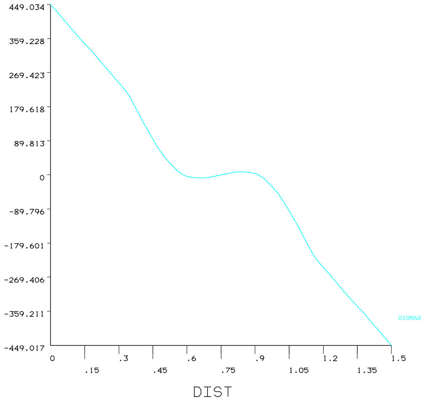
Stress concentration for beam with 2 central holes
