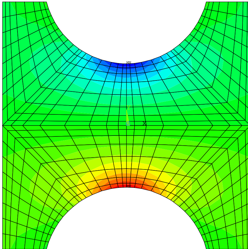
Notched Beam
