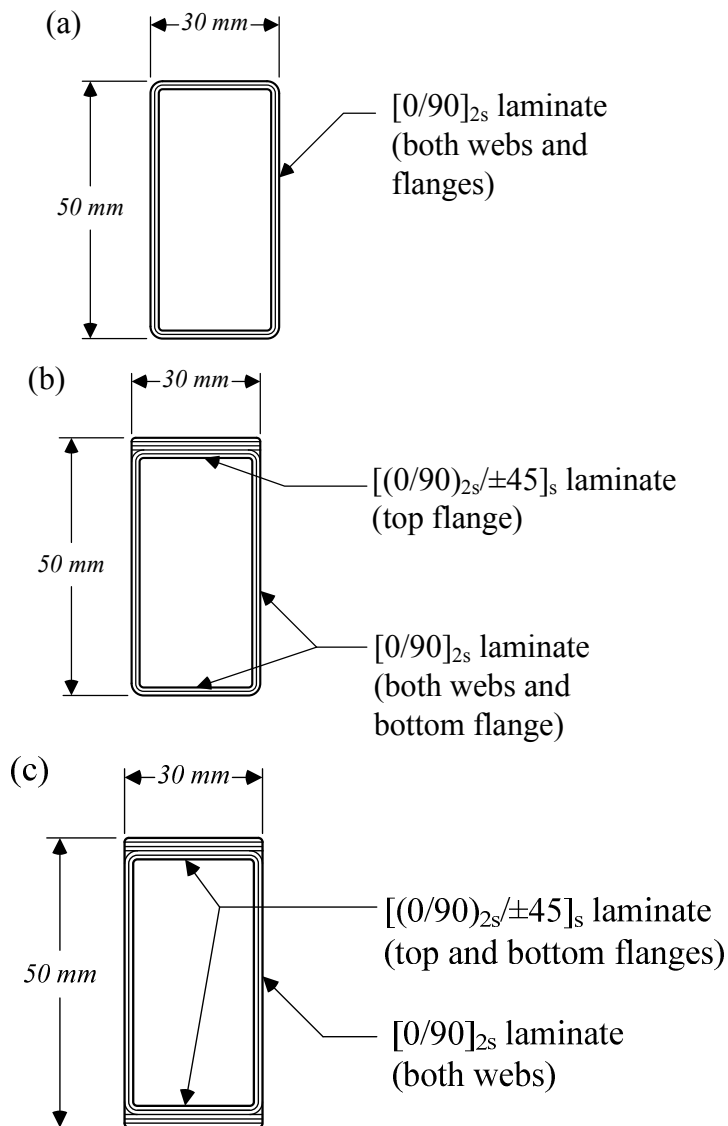
Figure 8.14: The composite box-beams considered in Example Problem 8.1 (not to scale). (a) Composite box-beam with identical stacking sequence in all web and flange laminates; (b) composite box-beam with additional plies added to the top flange laminate; (c) composite box-beam with additional plies added to both top and bottom flange laminates
