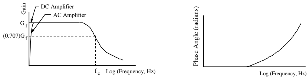
Figure 6: Idealized plot of typical amplifier gain and phase characteristics
