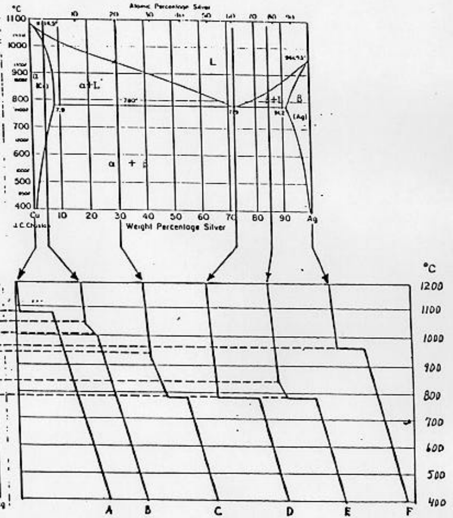
Figure 4. Equilibrium phase diagram showing relationship to cooling curves to the phase diagram for an eutectic alloy system.
