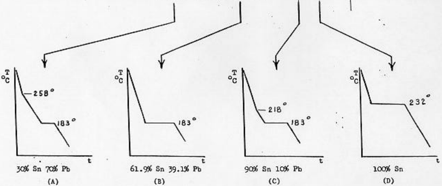
Figure 5. EXAMPLES OF COOLING CURVES FOR THE LEAD-TIN SYSTEM
