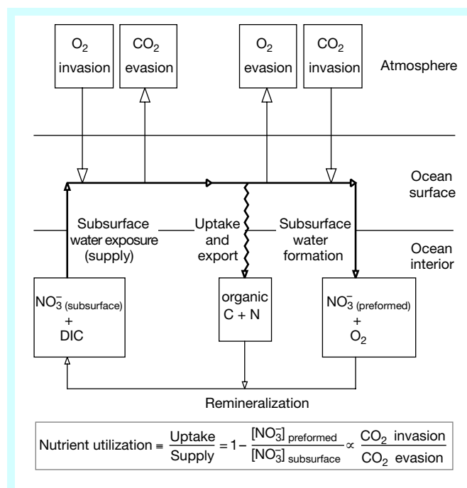
Figure 5 The effect on atmospheric \text{CO}_2 of the biological pump in a region of deep-ocean ventilation. Deep water is nutrient- and \text{CO}_2 -rich because of the lower-latitude biological pump, which sequesters both nutrients and inorganic carbon in the ocean interior; the major nutrients nitrate and phosphate are represented here as nitrate ( \text{NO}_3^- ) only. In high-latitude regions such as the Antarctic, the exposure of deep water at the surface releases this sequestered \text{CO}_2 to the atmosphere. However, the uptake of nutrients and \text{CO}_2 in the formation of phytoplankton biomass and the eventual export of organic matter subsequently lowers the p_{\text{CO}_2} of surface waters, causing the surface layer to reabsorb a portion of the \text{CO}_2 that was originally lost from the upwelled water. Thus, the ratio between export production and the ventilation of \text{CO}_2 -rich subsurface water, not the absolute rate of either process alone, controls the exchange of \text{CO}_2 between the atmosphere and high-latitude surface ocean. The nutrient concentration of water at the time that it enters the subsurface is referred to as its 'preformed' nutrient concentration. The preformed nutrient concentration of subsurface water provides an indicator of the cumulative nutrient utilization that this water underwent while at the surface, with a higher preformed nutrient concentration indicating lower cumulative nutrient utilization at the surface and thus a greater 'leak' in the biological carbon pump. The global efficiency of the biological pump can be evaluated in terms of the global mean preformed nutrient concentration of the ocean interior. In the calculation of this mean preformed nutrient concentration, each subsurface water formation term is weighted according to the volume of the ocean that it ventilates, because this corresponds to the amount of \text{CO}_2 that could be sequestered in a given portion of the ocean interior. As a result, surface ocean regions that are important in the ventilation of the ocean interior, such as the Antarctic, have particular importance for atmospheric \text{CO}_2 . This simple view overlooks some important facts. For instance, ocean/atmosphere \text{CO}_2 exchange is not instantaneous 68 , and variations in the chemical composition of export production also affects the p_{\text{CO}_2} of surface waters, as does sea surface temperature.
