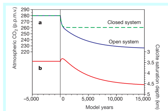
Figure 4 The time-dependent response of the CYCLOPS model to a sudden halving in the \text{CaCO}_3/\text{C}_{\text{org}} ratio of the export flux out of the low-latitude surface ocean 33 . The low-latitude surface ocean comprises the equatorial, tropical and subtropical oceans. a , Atmospheric \text{CO}_2 , for both 'closed' and 'open' system cases. b , Depth of calcite saturation (and the lysocline) in the open-system case. In the closed-system case, all of the \text{CaCO}_3 rain is dissolved in the ocean subsurface, with no burial, and there is no continental source of dissolved \text{CaCO}_3 . In the open-system case, which is more realistic, \text{CaCO}_3 is buried on the deep sea floor, and there is a continental input of dissolved \text{CaCO}_3 . The closed-system output has been offset to start at the same initial p_{\text{CO}_2} as the open-system case (280 p.p.m.v.). The closed-system effect of the \text{CaCO}_3/\text{C}_{\text{org}} rain ratio decrease is to extract less alkalinity from the surface ocean, which causes a 20 p.p.m.v. decrease in atmospheric \text{CO}_2 within hundreds of years. In the open-system case, the \text{CaCO}_3/\text{C}_{\text{org}} rain ratio decrease causes \text{CaCO}_3 burial to decrease below the input rate of alkalinity from the continents, both because of a transient dissolution event (evident as the early shoaling of the calcite saturation horizon, b ) and because of a permanent decrease in the \text{CaCO}_3 rain rate onto the sea floor. Due to both of these effects, ocean alkalinity increases, which causes the p_{\text{CO}_2} of surface water to decrease, so that atmospheric \text{CO}_2 decreases more in the open-system case than in the closed-system case ( a ). The whole-ocean alkalinity increase associated with the permanent decrease in the \text{CaCO}_3 rain rate, while contributing to the decrease in atmospheric \text{CO}_2 , also causes the deep-ocean carbonate ion concentration to increase through time, so that the calcite saturation horizon deepens. This deepening increases the area of sea floor on which \text{CaCO}_3 is preserved and buried so that global-ocean \text{CaCO}_3 burial increases back to equality with the river input of alkalinity, resulting in a new steady state with a deeper saturation horizon and lysocline. The model used here assumes that the carbonate ion concentration of deep water is the dominant control on the depth distribution of calcium carbonate burial in seafloor sediments (see text).
