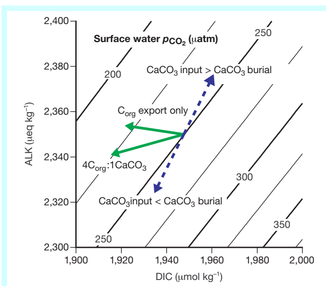
Figure 3 The p_{\text{CO}_2} of surface sea water at 20^\circ\text{C} and a salinity of 35 parts per thousand, as set by its dissolved inorganic carbon (DIC) content and alkalinity (ALK). The p_{\text{CO}_2} decreases as DIC decreases and/or ALK increases. The dashed arrows show the relative effects on ALK and DIC of imbalances in the \text{CaCO}_3 budget of the ocean. If \text{CaCO}_3 burial is less than the continental input of dissolved \text{CaCO}_3 , then the ALK and DIC of the whole ocean increase in a 2:1 ratio. This lowers the p_{\text{CO}_2} of surface waters and transfers \text{CO}_2 from the atmosphere into the ocean. The solid arrows show the effect of the rain of biogenic materials out of the surface ocean ('export production'), for the cases that this rain is organic carbon ( \text{C}_{\text{org}} ) only and that it is a 4:1 molar ratio of \text{C}_{\text{org}} and \text{CaCO}_3 . In general, the former composition applies to high nutrient polar surface ocean ecosystems, while the latter applies to the warm low-latitude ocean (references in ref. 98). Export production removes DIC from the surface ocean, sequestering it in the ocean interior. The modest ALK increase associated with \text{C}_{\text{org}} export only is due to the associated uptake of nitrate by phytoplankton. Export production also affects the DIC and ALK of the deep ocean, because \text{C}_{\text{org}} produced in the surface ocean and oxidized by bacteria in the ocean interior releases DIC and lowers the carbonate ion concentration of deep water. This affects the burial rate of \text{CaCO}_3 in the seafloor sediments, which further modifies the p_{\text{CO}_2} of surface waters through its effect on the whole-ocean \text{CaCO}_3 balance (dashed arrows).
