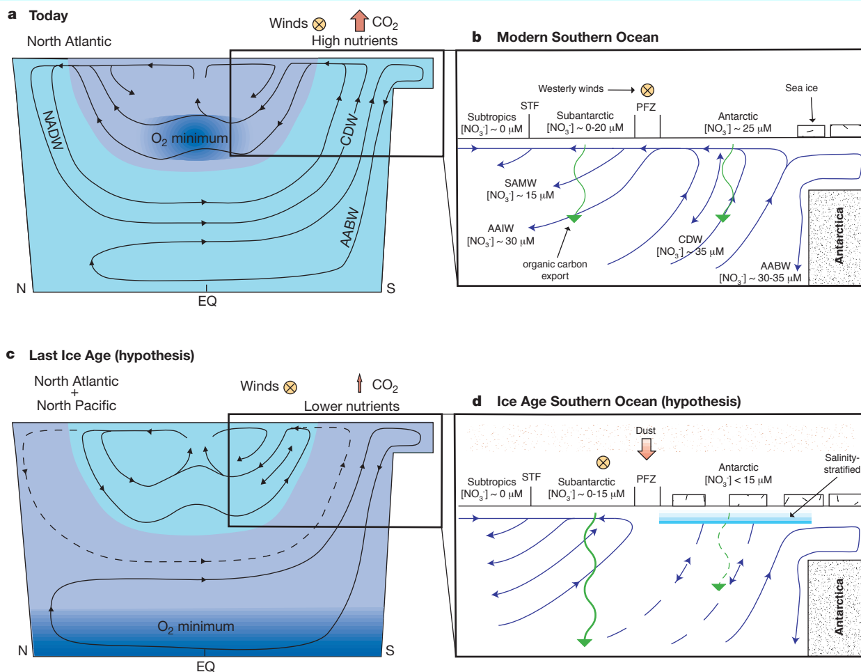
Figure 6 The modern ocean ( a, b ) and a Southern Ocean-based hypothesis for reduced levels of atmospheric CO 2 during glacial times ( c, d ). The figure shows a generalized depth section running from north to south ( a, c ) with an expanded view of the Southern Ocean ( b, d ). The north–south and vertical components of ocean circulation are shown (black flow lines in a and c , blue in b and d ). The blue shading in a and c indicates changes in the intensity of circulation between modern and ice-age times, with the lighter shade representing more vigorous circulation, illustrating the hypothesis that ice-age circulation was less vigorous in the cold, dense, deep ocean but more vigorous in the warmer, less dense, upper ocean. In the modern ocean ( a, b ), circulation of the interior can be characterized as follows. New deep water forms in the high-latitude North Atlantic (North Atlantic Deep Water, NADW). NADW flows south and mixes with other deep waters (including Antarctic Bottom Water, AABW) to generate Circumpolar Deep Water (CDW). Eastward winds (orange circled cross) over the Polar Frontal Zone (PFZ) drive upwelling of CDW into the Antarctic surface, releasing deep-sequestered CO 2 to the atmosphere (upward red arrow in a ). Antarctic surface water flows northward to the PFZ, where it sinks into the subsurface as Antarctic Intermediate Water (AAIW) or mixes with subantarctic surface water, some of which forms Subantarctic Mode Water (SAMW). The biological production and export of organic matter (green arrows) extracts nutrients and inorganic carbon from surface waters, causing the nitrate concentration ([NO 3 ]) of the Antarctic surface (~25 μM), the subantarctic surface (0–20 μM), and newly formed AAIW and SAMW (~30 and ~15 μM, respectively) to be lower than that of the CDW that was originally upwelled (~35 μM). AAIW and SAMW ventilate the mid-depth ocean and supply nutrients to the lower-latitude surface. This nutrient supply fuels biological export production, the degradation of which causes a subsurface deficit in dissolved oxygen which is most intense at intermediate depths (the O 2 minimum in a ). The hypothetical ice-age Southern Ocean described in the text includes the following changes ( c, d ). Upwelling into the Antarctic surface decreased, possibly due to an equatorward shift in the belt of eastward winds, and/or a freshening of the surface ('salinity-stratification') related to an increase in sea ice. In the subantarctic, the winds may have driven the upwelling of intermediate-depth waters, which formed in the North Atlantic and/or North Pacific. The supply of iron from dust was high (broad downward arrows and red stippling). Organic carbon export was higher in the subantarctic but lower in the Antarctic (green arrows). Possibly due to the greater supply of dust-borne iron, the degree of nitrate utilization was higher in both regions, leading to lower surface [NO 3 ] and less nutrient transport to the lower latitudes. This pattern of nutrient supply and export production caused the O 2 minimum to migrate into the abyssal ocean and reduced the release of CO 2 from the Southern Ocean.
