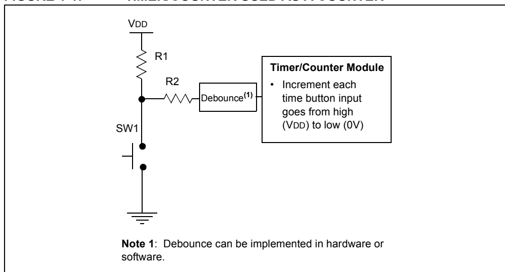
FIGURE 1-1: TIMER/COUNTER USED AS A COUNTER
