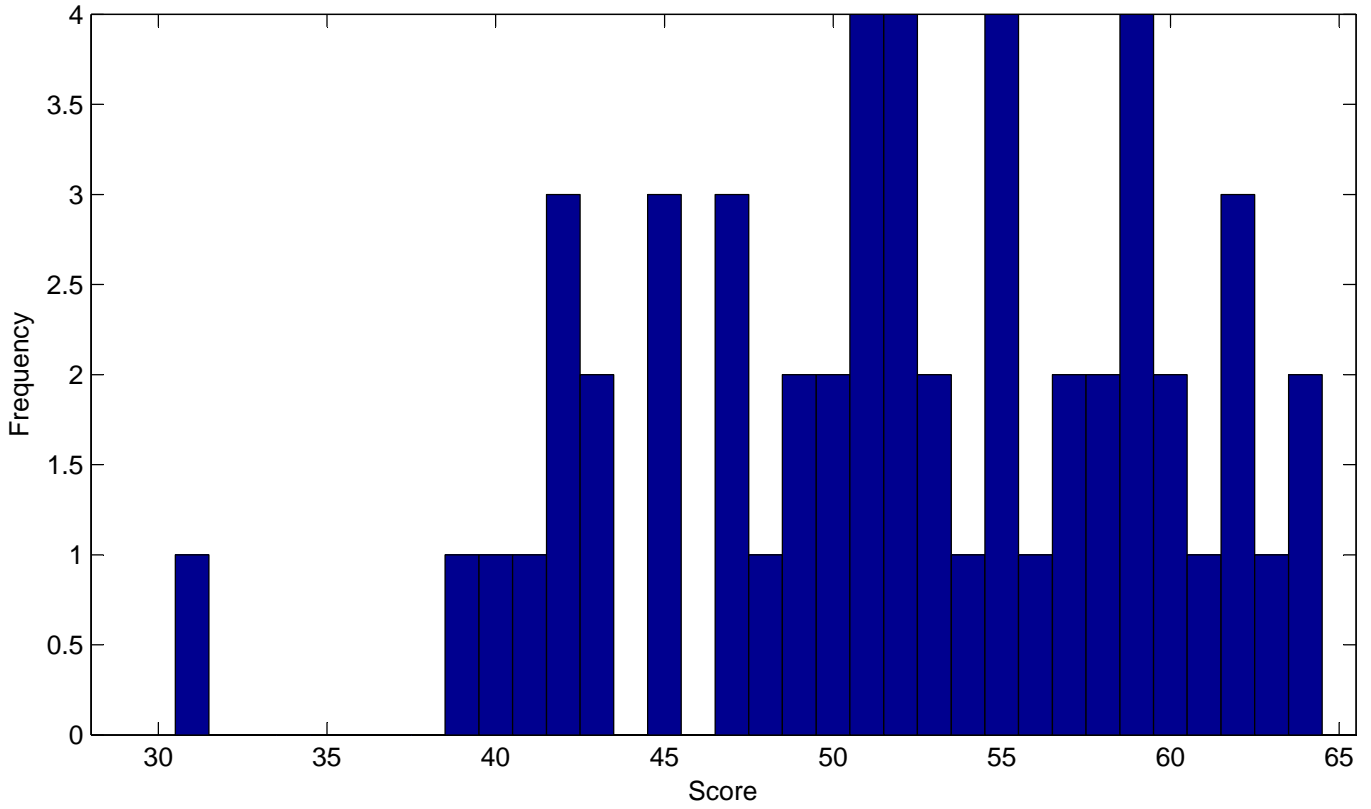
Final Exam Scores, median 52 out of 65
