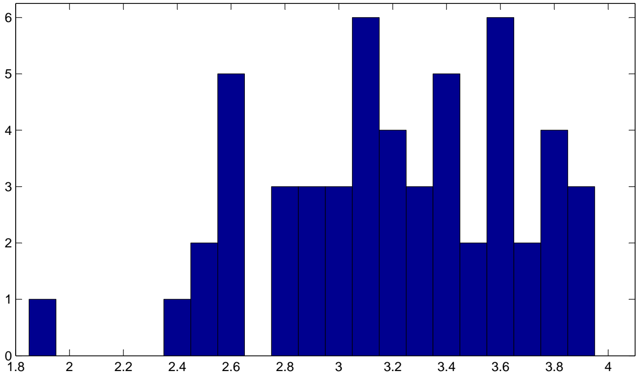
Grades( 4 \times \text{Scores} / 65 ), median 3.2
