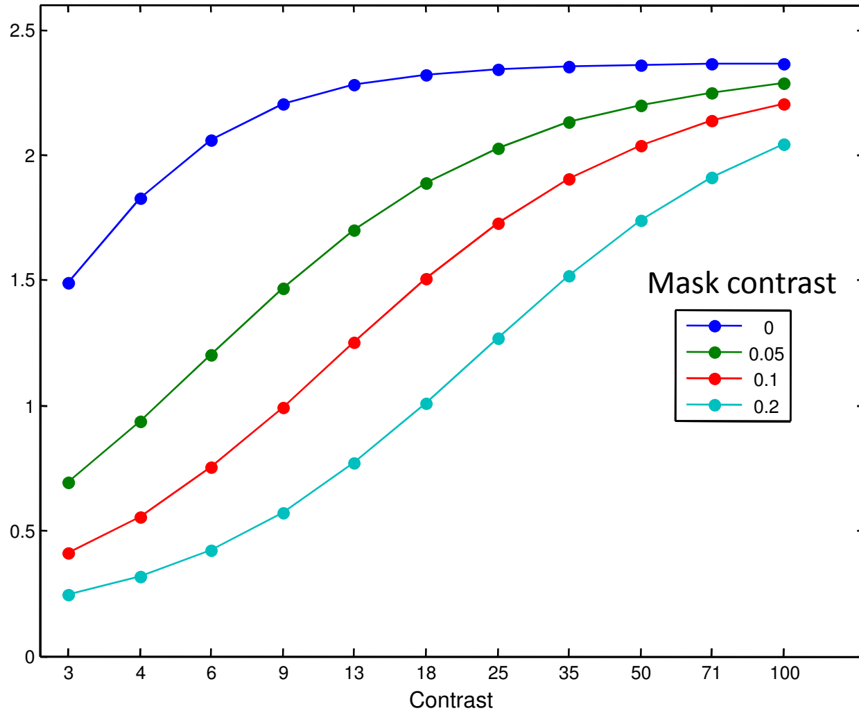
Contrast-dependence on cross-orientation suppression
