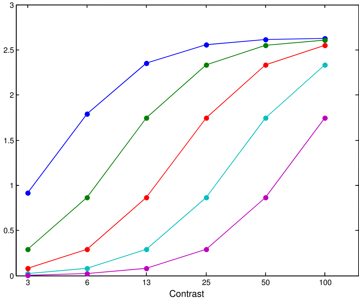
Effects of adaptation on contrast-response functions
