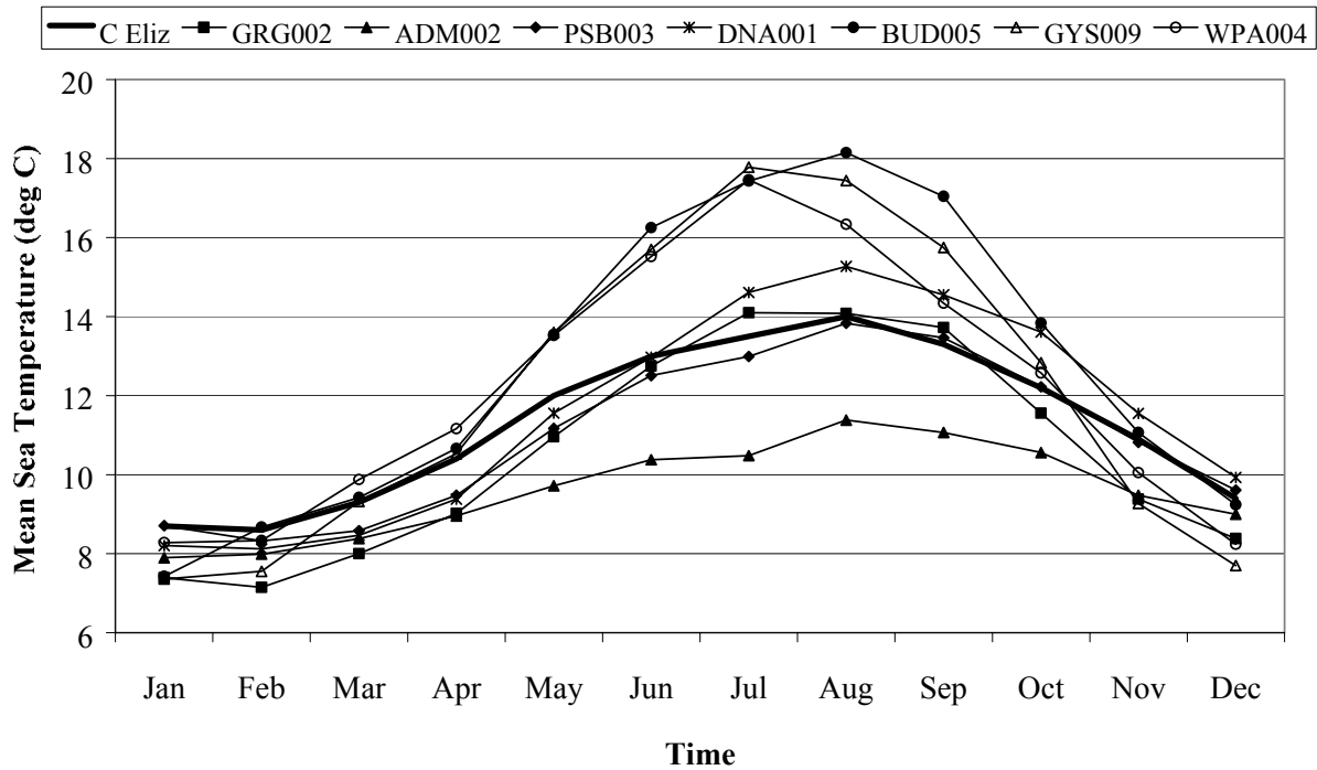
Figure 6. Sea-Surface temperature long-term means for several Ecology monitoring stations and for the NOAA Cape Elizabeth National Data Buoy. Long-term means for Ecology data are from monthly values from WY 1990 - Y 2000; long-term means for Cape Elizabeth data buoy are from hourly values from June 1987 - December 2001, as presented on the NOAA National Data Buoy Center website ( www.ndbc.noaa.gov ).
