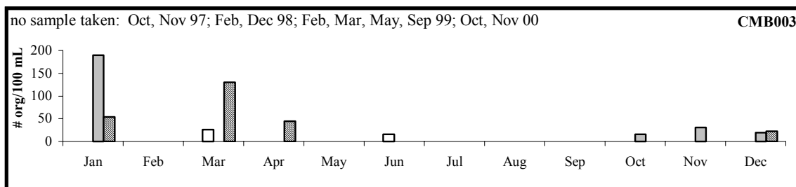
Figure 17. Fecal coliform bacteria concentrations versus calendar month for stations with high counts (> 14 organisms/100mL) during WY 1998 – Y 2000.
