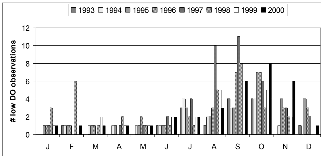
Figure 12. Number of observations in a given month of dissolved oxygen concentrations <5 mg/L for years 1993 through 2000. All data transformed to calendar year for this figure.
