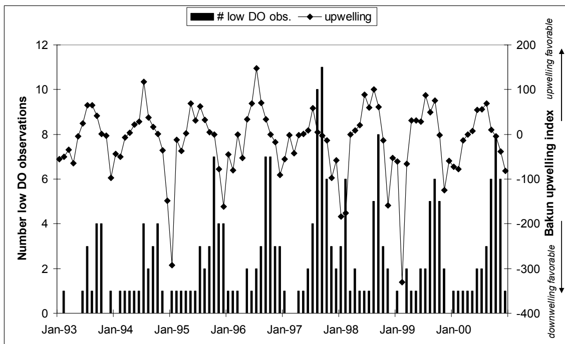
Figure 11. Number of observations of dissolved oxygen concentrations <5 mg/L at core stations and the Bakun upwelling index at 48^{\circ} N, 125^{\circ} W for 1993 through 2000. Note that the number of observations in a given month can be biased due to missing flights, see text.
