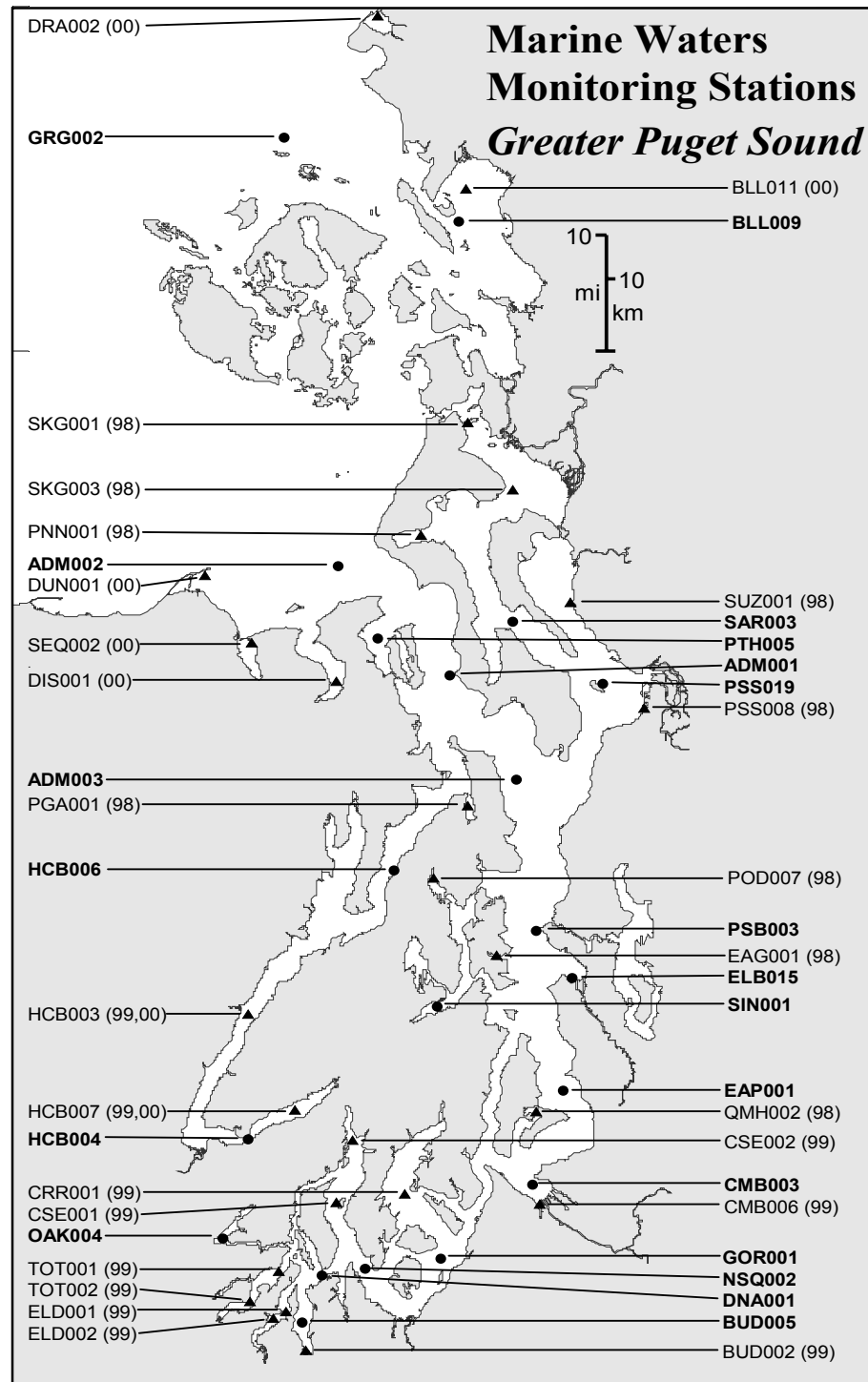
Figure 1. Marine Waters Monitoring stations in Puget Sound for WY 1998 – Y 2000. Rotational stations (triangles) are shown with the year sampled in parentheses. The core stations (circles) are sampled every year.
