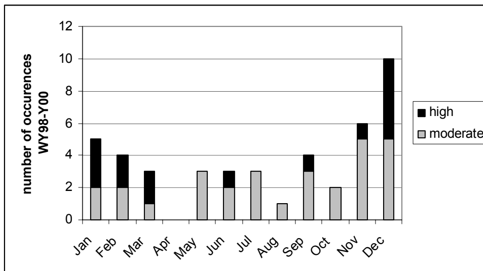
Figure 19. Annual distribution of the occurrences of high or moderate fecal coliform bacteria counts recorded during WY 1998 through Y 2000 for a) Puget Sound and b) Grays Harbor and Willapa Bay.
