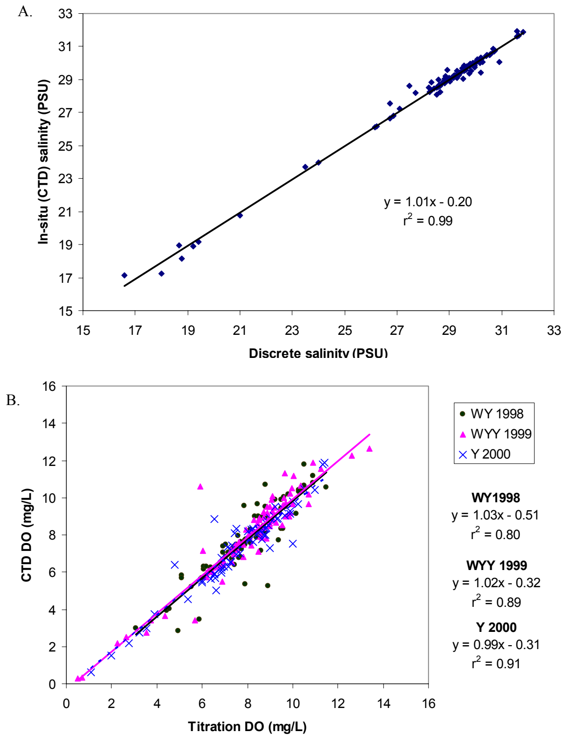
Figure 20. Comparisons of sensor versus discrete sample measurements. A. Regression of CTD sensor-derived salinity versus that from discrete samples. Data shown are composited samples for WY 1998-Y 2000. B. Regression of CTD sensor versus titration results for DO sensor verification samples collected in WY 1998, WYY 1999 and Y 2000.
