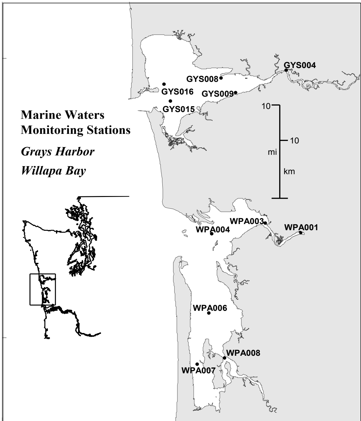
Figure 2. Marine Waters Monitoring stations for WY 1998 – Y 2000 in Grays Harbor and Willapa Bay. All stations are core stations.
