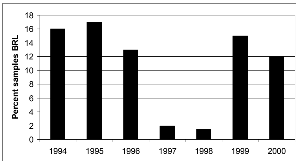
Figure 13. The percent nutrient samples collected with below-reporting-limit concentrations of nitrate+nitrite-N. Data for 1994 through 1998 represent wateryears; 1999 and 2000 follow the convention used in this report (WYY 1999 and Y 2000).
