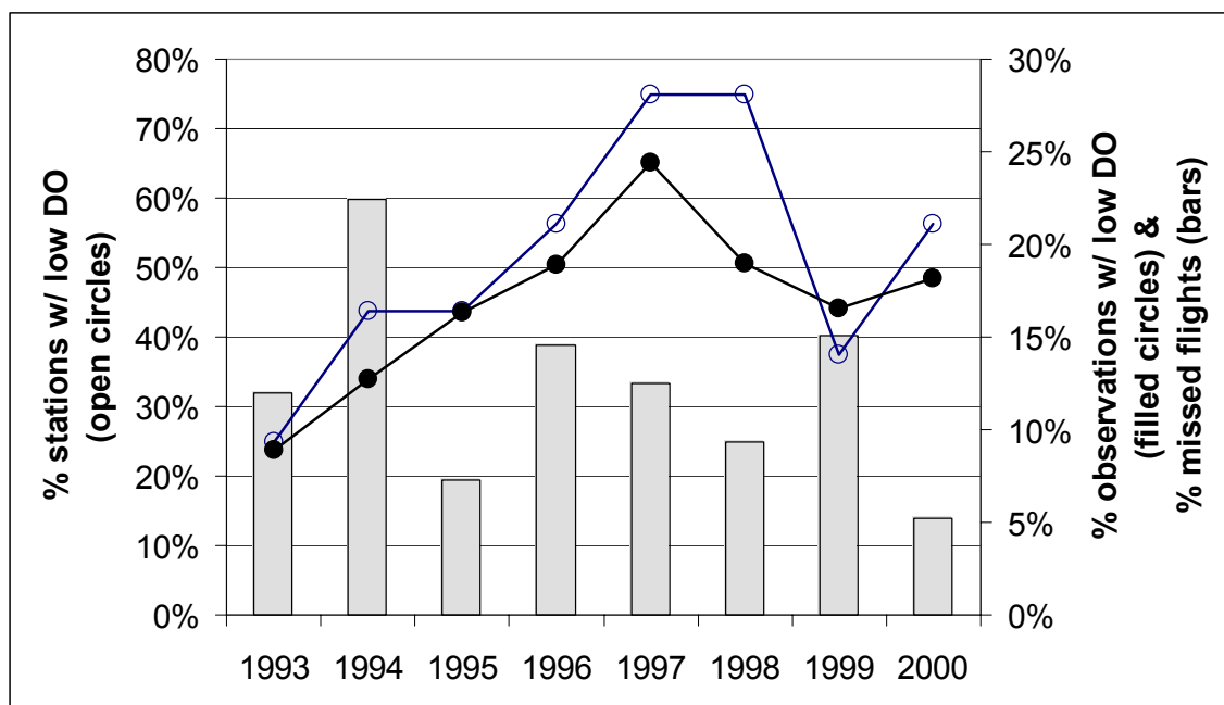
Figure 10. Occurrence of low dissolved oxygen (<5 mg/L) from WY 1993 – Y 2000. Shown is the percent of stations with low DO (open circles) as well as the % of the observations with low DO (filled circles). The percent of missed observations in a given year is shown by the bar.
