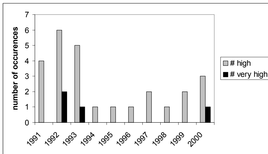
Figure 15. Number of observations of high (>5 µM) and very high (>10 µM) ammonium-N concentrations in central Budd Inlet at BUD005 since WY 1991. Nitrogen removal from LOTT effluent began in early 1994.
