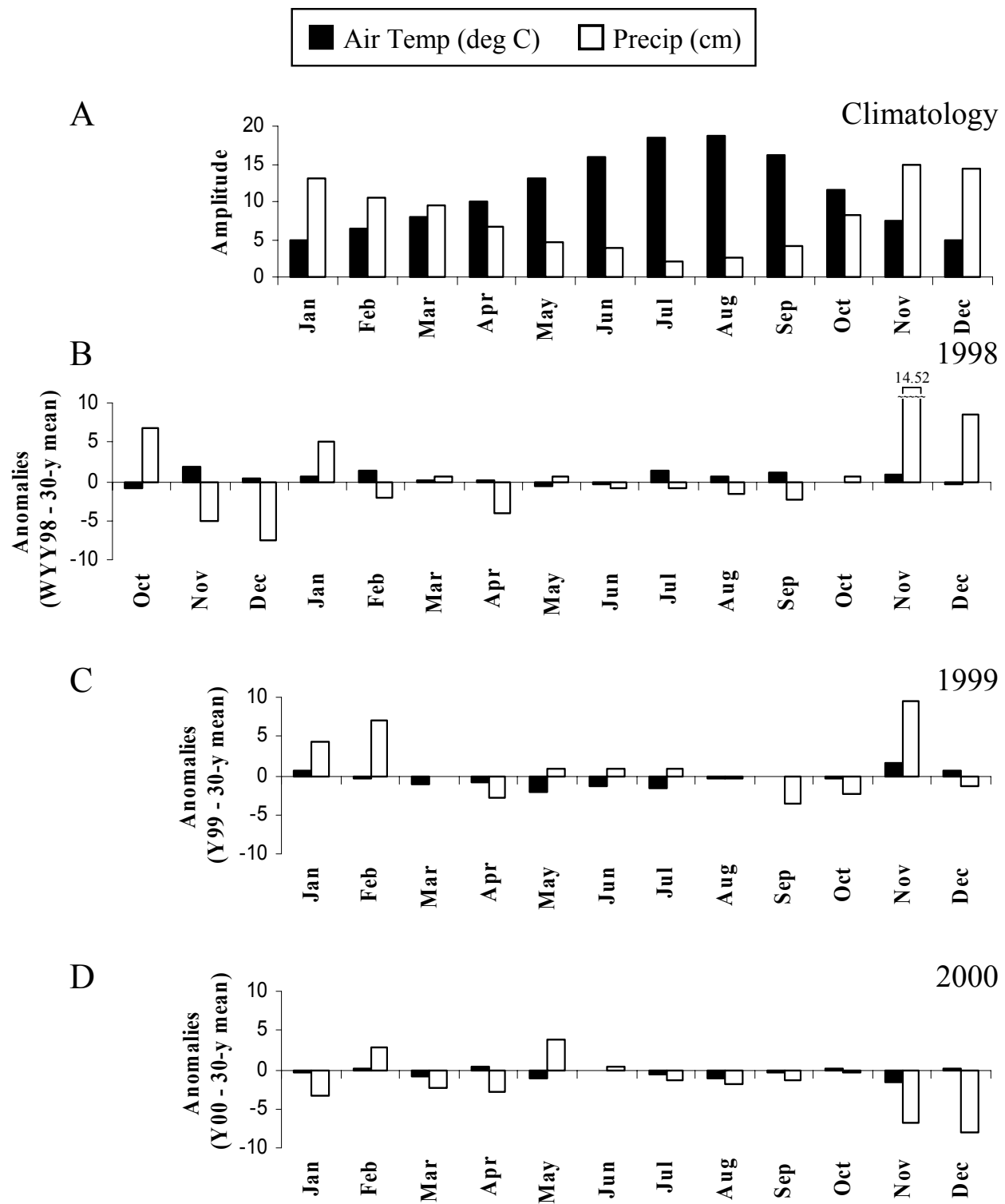
Figure 3. Climate data for WYY 1998, Y 1999, and Y 2000. (A) Climatology (30 year-mean, 1971-2000). (B, C, D) Anomalies for WYY 1998, Y 1999, and Y 2000 air temperatures and precipitation compared to 30-year average. Data obtained from the Western Regional Climate Center ( http://www.wrcc.dri.edu/ ) for Sea-Tac Airport.
