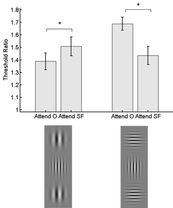
Figure 3. Experiment 2 results. Postadaptation threshold ratios for the two adapting stimulus conditions as a function of attended dimension. Error bars depict standard errors. Threshold ratios were significantly lower for both stimulus conditions when attention was directed to the feature dimension that was the same than to the dimension that differed. (SF: spatial frequency; O: orientation; *: p < 0.05 ).
