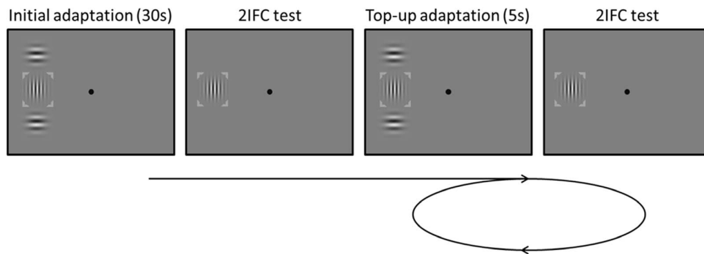
Figure 1. Contrast adaptation experimental procedure. Observers were initially presented with the adapting stimuli for 30 s (counter-phase flickering at 2 Hz), followed by the first 2IFC detection trial (see Methods). Each subsequent 2IFC trial was preceded by 5 s of the adapting stimuli (counter-phase flickering at 2 Hz). The attention tasks were confined to the initial and top-up adaptation periods.
