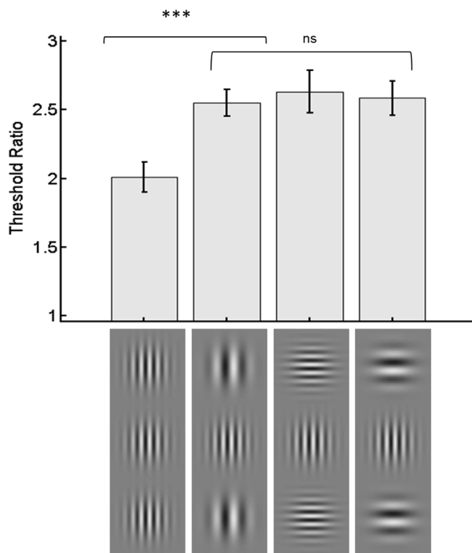
Figure 2. Experiment 1 results. Postadaptation threshold ratios for each adapting stimulus condition. Error bars depict standard errors. Threshold ratios were significantly lower for the same spatial frequency/same orientation adapting stimulus than for the other three stimulus conditions, which did not differ from one another. ***: p = 0.002 ; ns = not significant.
