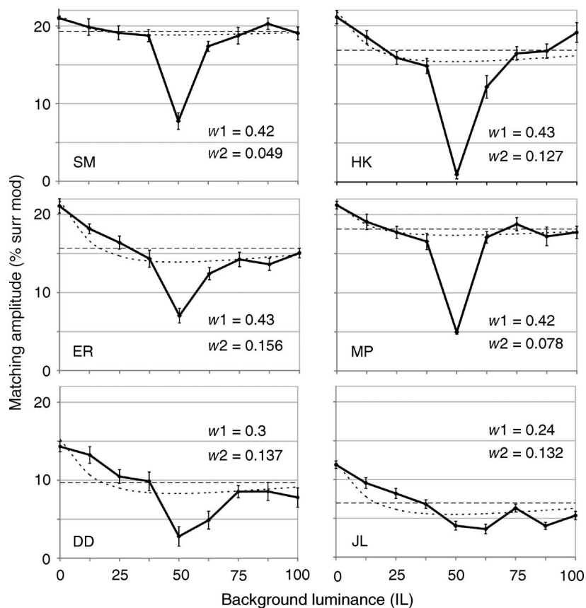
Figure 6. The individual data (black diamonds/solid lines) are fit by Extended Weighted Michelson Contrast model (dotted lines), and by Extended Weighted Log Luminance Ratio model (dashed lines). The individual weights for Extended Weighted Michelson Contrast model are given within each panel. All the conventions are the same as in Figure 5 .
