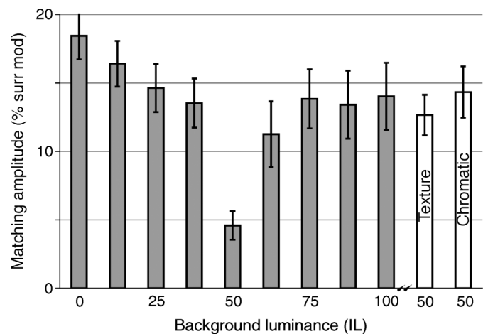
Figure 4. Average induction effects for two experiments. Background luminance is plotted along the abscissa, in instrument luminance (IL) units. Matching induction amplitude is plotted along the ordinate, in percent of surround modulation amplitude. Each bar represents the induction effect on the particular background, averaged for 6 subjects. The error bars show the standard error of the mean.
