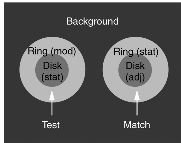
Figure 1. The stimulus. A temporally static test disk is presented on the left, surrounded by a temporally modulated ring. An adjustable disk (“match”) is presented on the right, surrounded by a static ring. The amplitude of luminance modulation of the match disk can be changed by the observer to match the perceived lightness change in the test disk. The disk/surround combinations are presented on backgrounds, which differed in luminance (Experiment 1); chromaticity and texture (Experiment 2).
