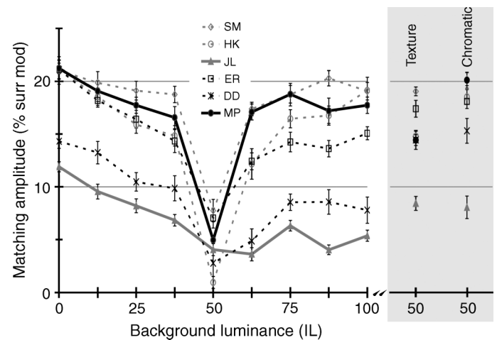
Figure 3. Main graph: Induction effect as a function of background luminance ( Experiment 1 ). Background luminance is plotted along the abscissa, in instrument luminance (IL) units. Matching induction amplitude is plotted along the ordinate, in percent of surround modulation amplitude. Each curve in the graph represents one subject's induction effect measured on different backgrounds. The error bars show the standard error of the averaged match values. Inset on the right: Induction effect as a function of background texture and chromaticity ( Experiment 2 ). All conventions are the same as in the main graph.
