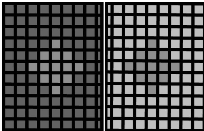
Figure 7. The dungeon illusion. The diamond-like configuration of square patches on the left-hand side appears to be lighter than that on the right-hand side, even though they have the same luminance.
