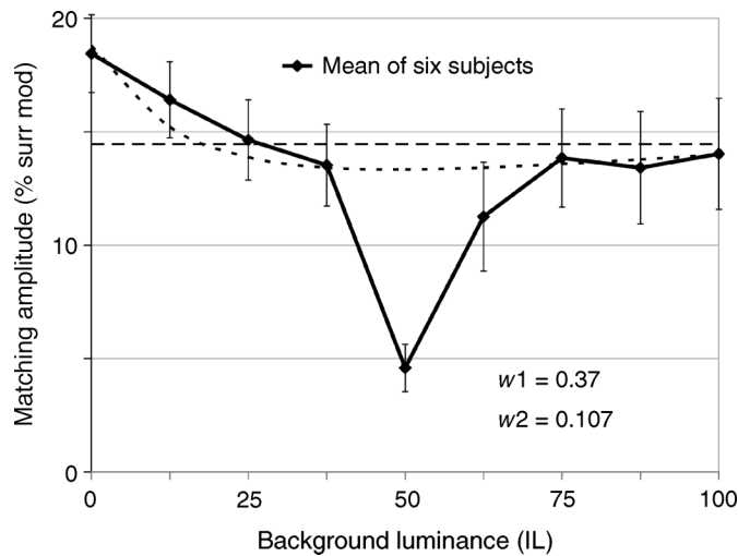
Figure 5. The averaged data of six subjects (black diamonds/ solid line) are fit by Extended Weighted Michelson Contrast model (shown by the dotted lines), and by Extended Weighted Log Luminance Ratio model (shown by the dashed lines). The values of w_1 and w_2 represent the relative influences (or weights) of the disk/ring and the ring/background luminance borders of Extended Weighted Michelson Contrast model . All the conventions are the same as in Figure 3 .
