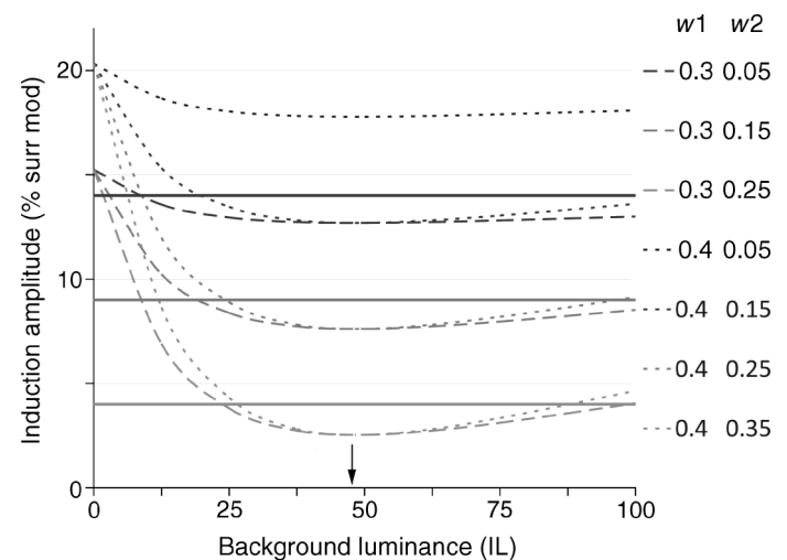
Figure 2. Predictions of two extended models. The predictions of the Extended Weighted Michelson Contrast model are shown by dashed and dotted lines. Different lines show the nested models for different w_1 and w_2 weight combinations (the respective weights are specified by the first and the second number in the Legend). An arrow shows predicted minimum. The predictions of the Extended Weighted Log Luminance Ratio model are shown by solid lines. Since there are multiple weight combinations resulting in the same predictions, the particular weights are not specified for this model. Background luminance is plotted along the abscissa, in instrument luminance (IL) units. Predicted induction amplitude is plotted along the ordinate, in percent of surround modulation amplitude.
