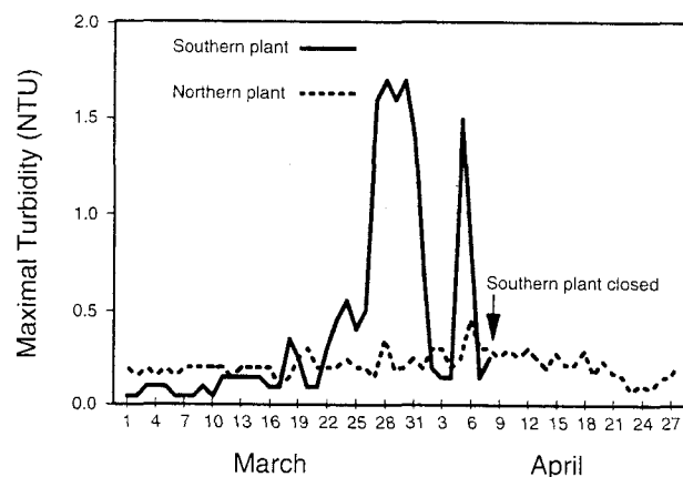
Figure 1. Maximal Turbidity of Treated Water in the Northern and Southern Water-Treatment Plants of the Milwaukee Water Works from March 1 through April 28, 1993.
